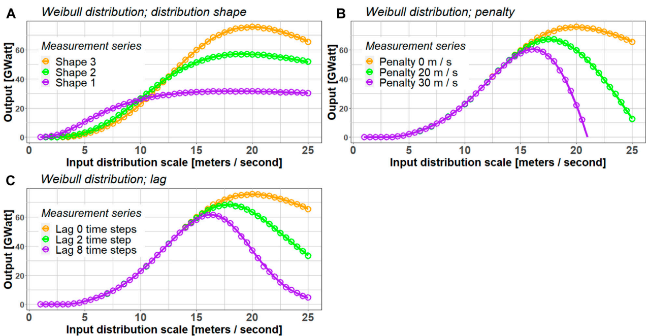
FIGURE 6 Output wind power as a function of the scale of the wind speed input distribution under changing (A) distribution shape (distribution shape k = 1 to 3 ; penalty p = 0 meters / second; lag l = 0 time steps), (B) penalty size (distribution shape k = 3 ; penalty p = 0 to 30 meters / second; lag l = 0 time steps), and (C) lag duration (distribution shape k = 3 ; penalty p = 0 meters / second; lag l = 0 to 8 time steps) for the Weibull distribution; for each set of parameters the results of the minimal models (continuous lines) and the simulations (circles) are presented; the power values (y-axis) were obtained by assuming an air density of \rho = 1.225\text{kg/m}^3 and a rotor blade radius of r = 100 m.
