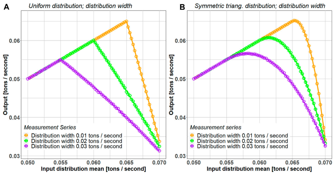
FIGURE 5 Output mass flow as a function of the mean of the mass flow input distribution for various input distribution widths for the (A) uniform distribution (distribution width w = 0.01 to 0.03 tons/second; penalty p = 0.00 tons/second; lag l = 0 time steps) and the (B) symmetric triangular distribution (distribution width w = 0.01 to 0.03 tons/second; penalty p = 0.00 tons/second; lag l = 0 time steps); for each set of parameters the results of the minimal models (continuous lines) and the simulations (circles) are presented.
