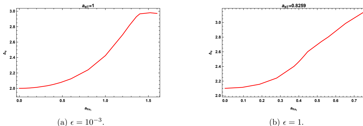
Figure 2. Maximizing the gap in the singlet sector with varying the OPE coefficient a_{tt\phi_1} with fixed a_{ttT} .
