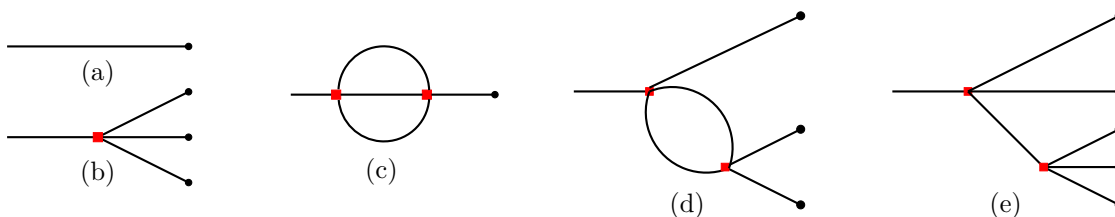
Figure 1. Feynman digrams for \langle \phi_1(\tau, \vec{x} = 0) \rangle upto O(g_1^2, g_2^2, g_1 g_2) . The filled red square denotes the bulk couplings whereas the filled circle denotes the defect coupling.
