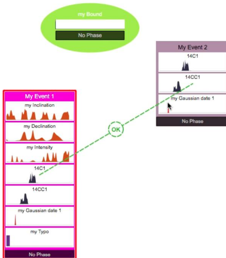
Figure 49: Events scene showing a constraint between 2 Events
