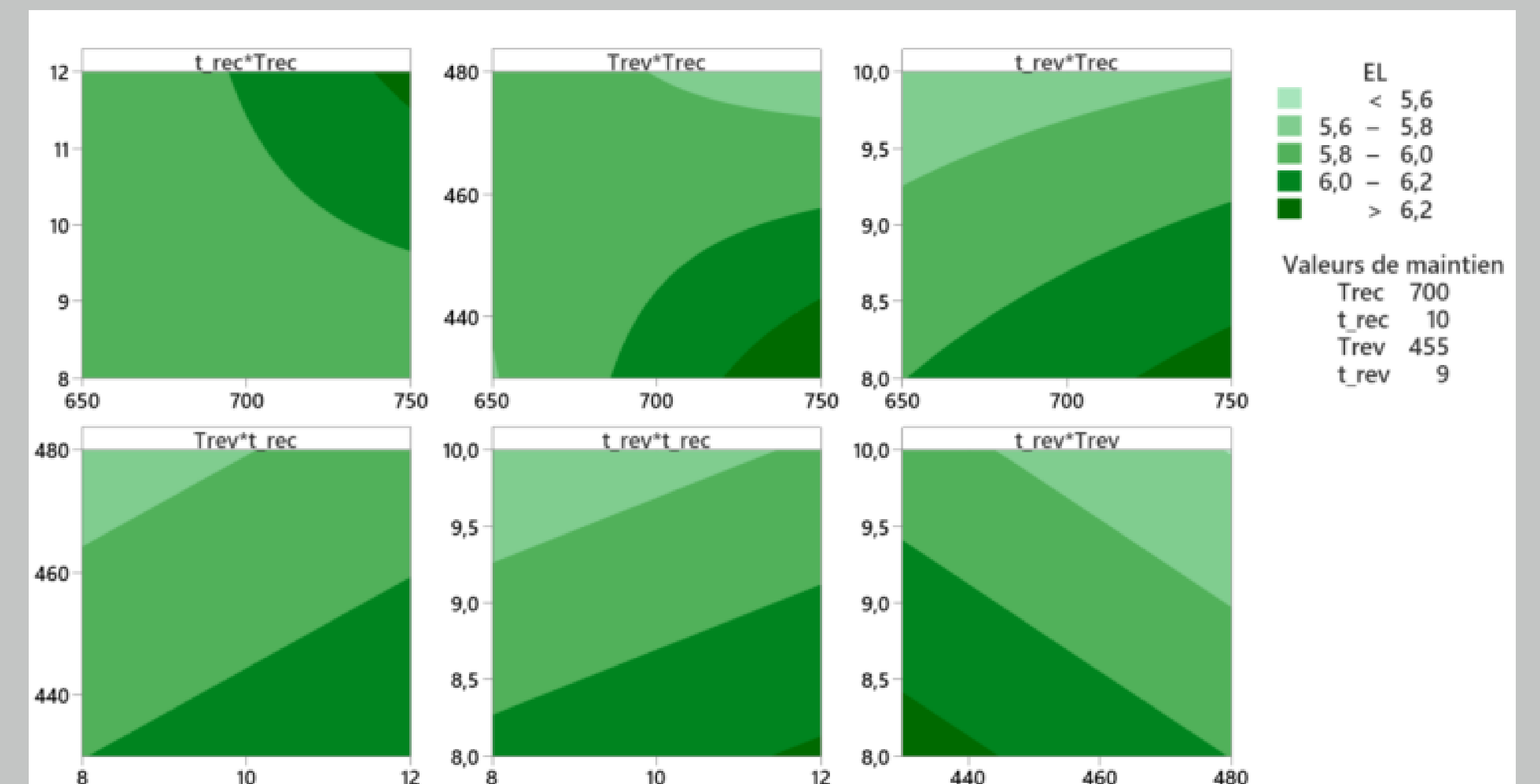
Figure 2: Contour plots of \epsilon_L
