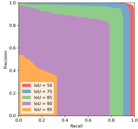
Figure 7: P-R curve for Model B (CV test subset #2). The \mathbf{AP}^\Theta figures in table 3 correspond to the area under the curves (displayed in colors)
