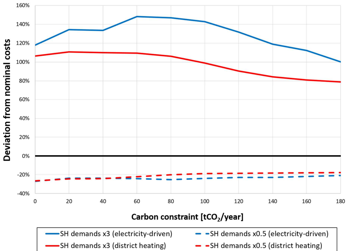
Figure 9. Sensitivity of both architectures to variations in space heating demands.
