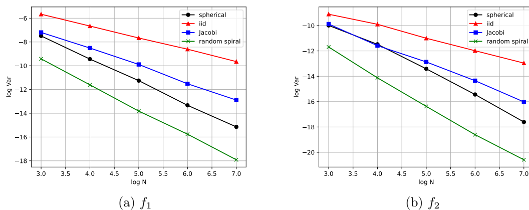
Figure 4: log variance of four integral estimators wrt. the number N of quadrature nodes.
