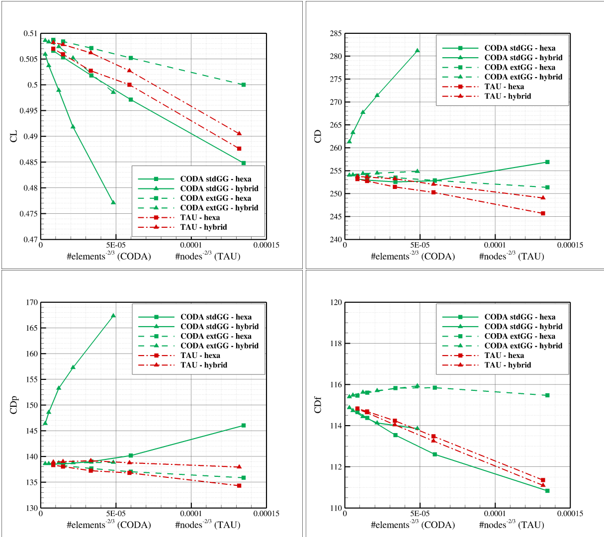
Fig. 8 C_L (top left), C_D (top right), C_{D_p} (bottom left) and C_{D_F} (bottom right) coefficients for the mesh convergence study related to the DPW-5 CRM configuration. CODA stdGG and extGG results are compared to the reference TAU solutions.
