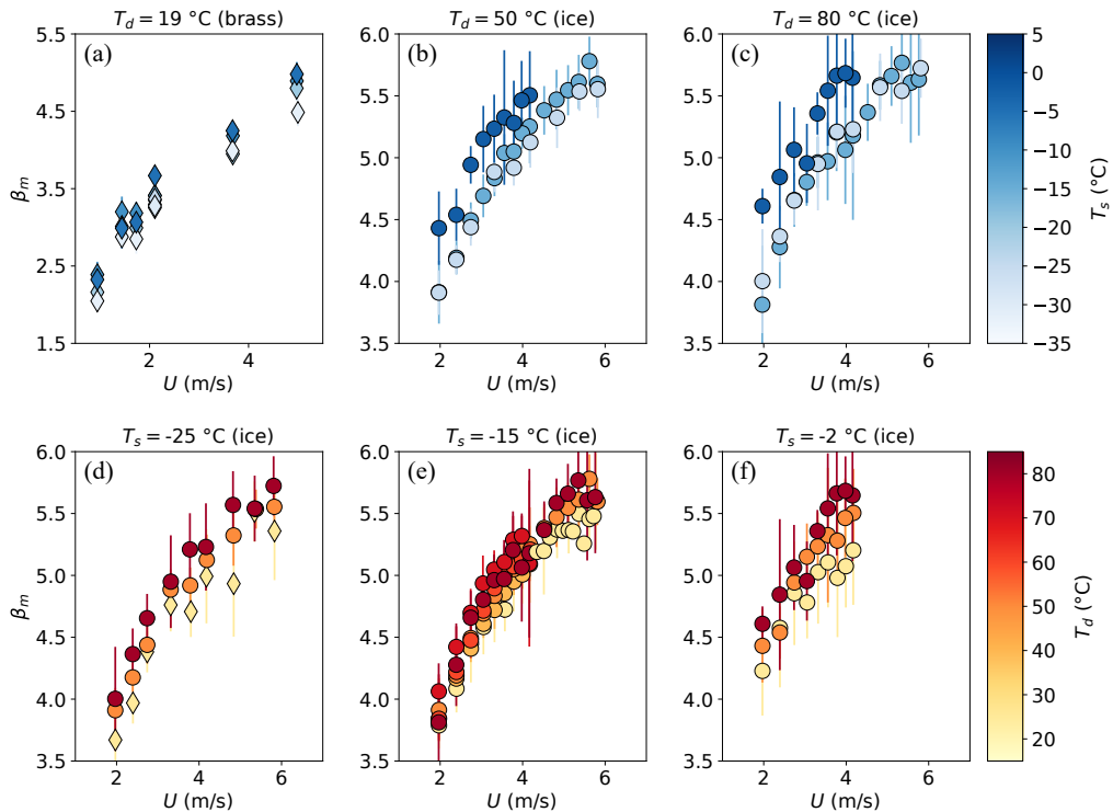
Figure 2: Evolution of the maximum spreading ratio \beta_m \equiv D_{\min}/D_0 , as a function of the impact velocity U . In (a)-(c), the droplet temperature is fixed at (a) T_d = 19^\circ\text{C} (brass), (b) T_d = 50^\circ\text{C} (ice), and (c) T_d = 80^\circ\text{C} (ice), while the colorbar denotes the substrate temperature T_s . Contrariwise, in (d)-(f) the substrate temperature is fixed at (d) T_s = -25^\circ\text{C} (ice), (e) T_s = -15^\circ\text{C} (ice), and (f) T_s = -2^\circ\text{C} (ice), while the markers' colours represent this time the droplet temperature T_d . The symbols correspond to experiments with ( \diamond ) solidification or ( \circ ) fusion, respectively. The nature of the substrate is indicated above each plot.
