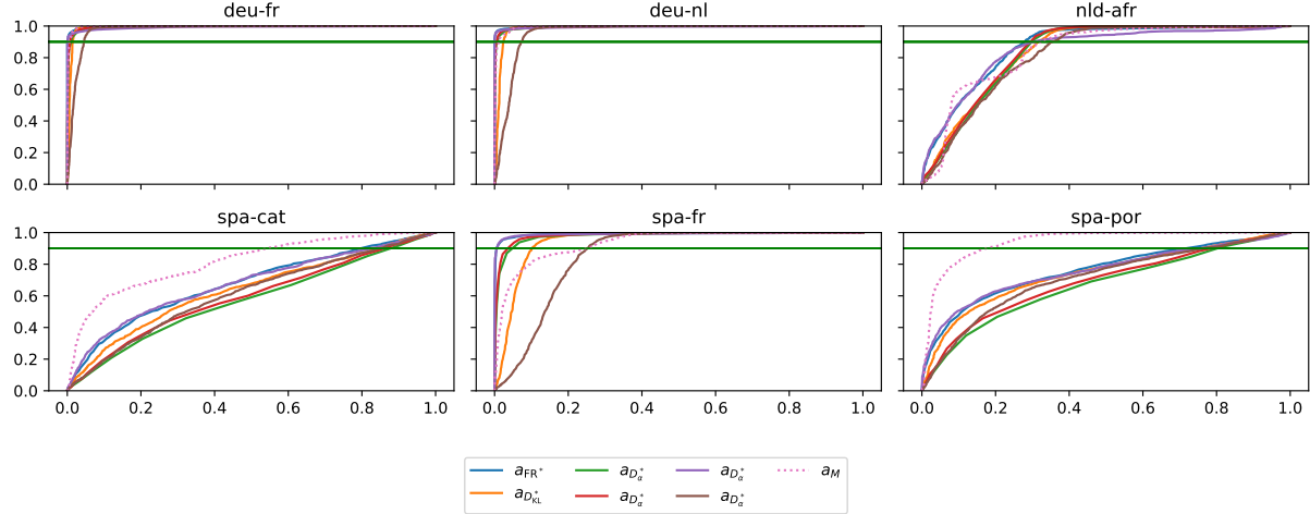
Figure 8: ROC-AUC curves for our reference-based metrics compared to common baselines for language shift detection. Baselines are represented in dashed lines.
