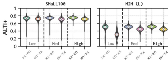
Figure 3: Distribution of SMaLL100 and M2M (L) ALTI+ scores for en-xx and xx-en directions.
