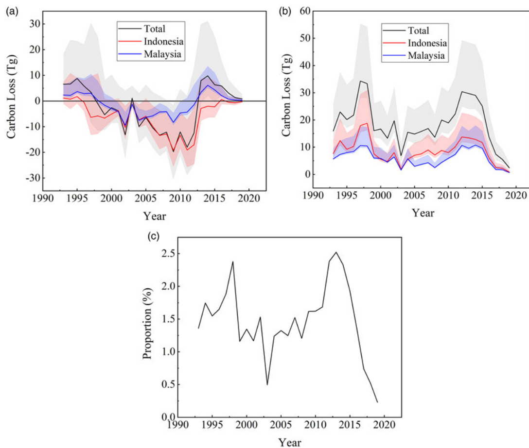
Figure 5. The characteristics of changes in carbon stocks. (a) Total carbon emissions caused by oil palm expansion. (b) Carbon emissions from the invasion of forests by oil palm plantations. (c) The ratio of carbon emissions resulting from oil palm plantation expansion into forests to global carbon emissions caused by land use change (Friedlingstein et al. 2022).
