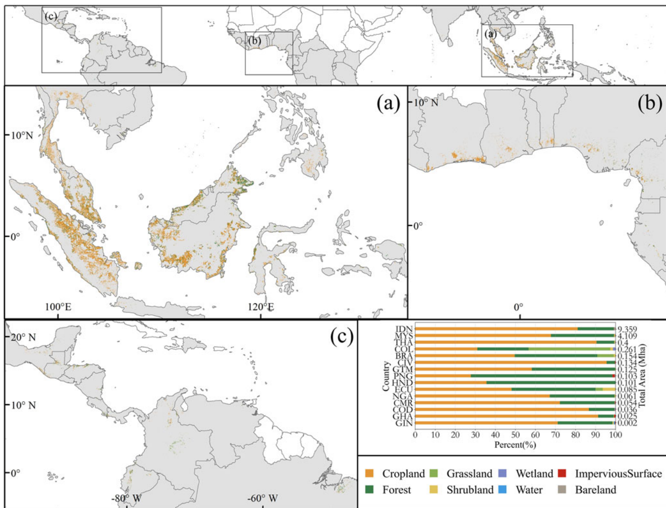
Figure 2. Land conversion by oil palm plantations in various countries. The stacked bar chart depicts the expansion of oil palm plantations from 1992 to 2019 in 15 countries. These countries are the ones for which oil palm sample data are available. BRA, Brazil; ECU, Ecuador; COL, Colombia; GTM, Guatemala; HND, Honduras; GIN, Guinea; GHA, Ghana; COD, the Democratic Republic of the Congo; CMR, Cameroon; CIV, Ivory Coast; NGA, Nigeria; THA, Thailand; MYS, Malaysia; IDN, Indonesia; PNG, Papua New Guinea.
