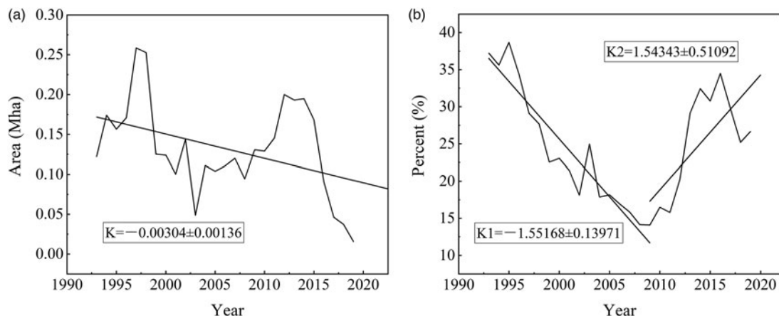
Figure 4. The characteristics of oil palm plantation expansion into forest. (a) The area of forest was converted to oil palm plantations. (b) The proportion of forest covered by oil palm plantations.
