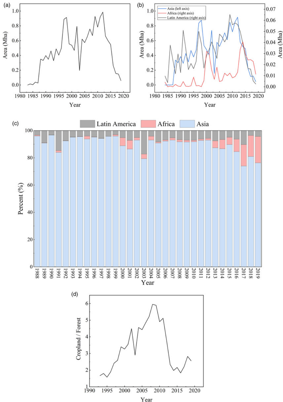
Figure 3. The characteristics of oil palm expansion. (a) Global annual expansion of oil palm plantations. (b) Continental expansion of oil palm plantations, including Asia (left Y axis), Africa (right Y axis), and Latin America (right Y axis). (c) The percentage of oil palm plantation expansion areas in each continent relative to the total expansion area for each year. (d) The ratio of converted agricultural land to forest area is a critical measure.
