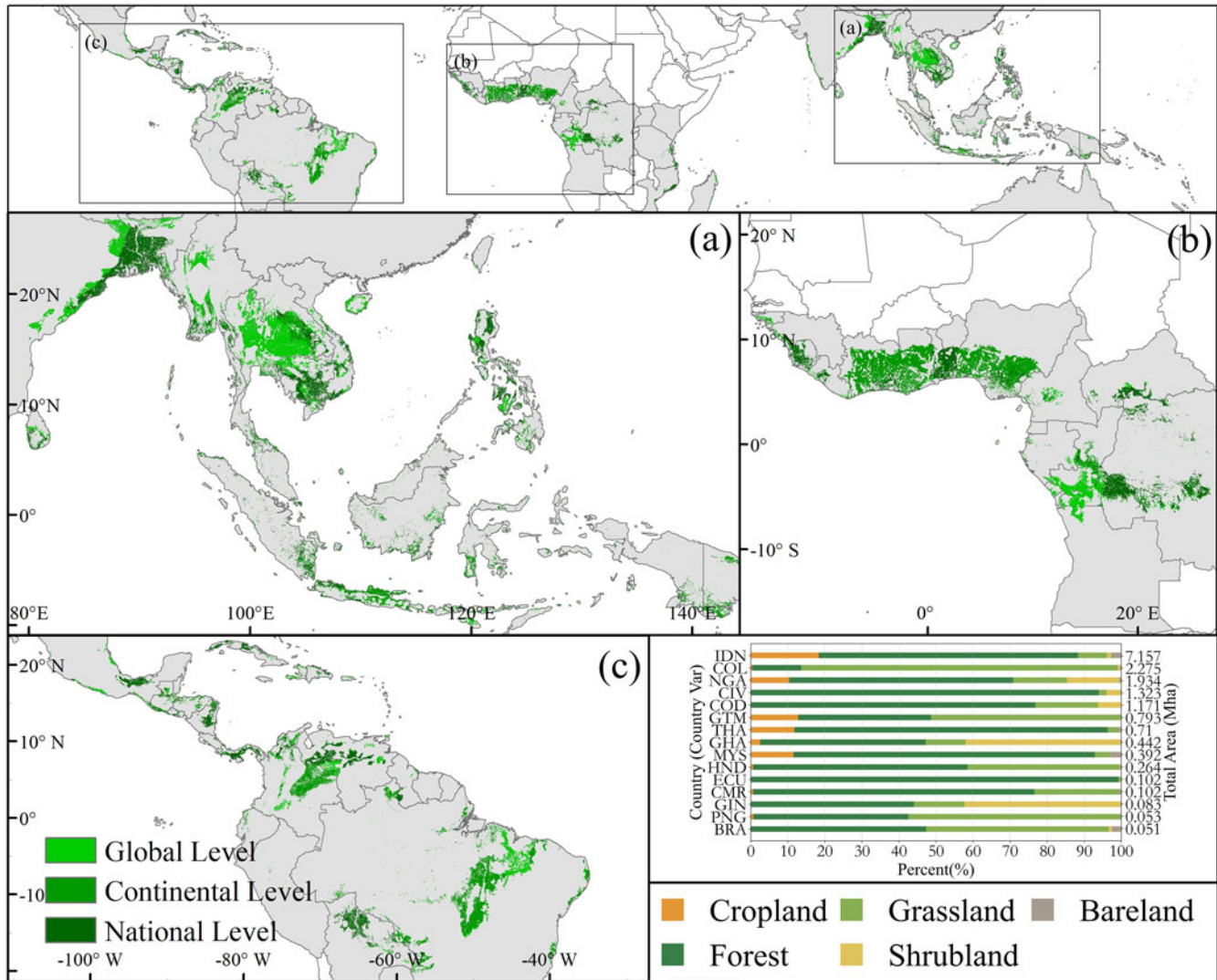
Figure 6. Potentially available land for oil palm expansion at global, continental, and national levels under different restrictions. Unconvertible areas (wetlands, water bodies, and urban areas), peatland, protected areas, and high biomass density areas were excluded from the potentially available land. The stacked bar chart illustrates the potentially available land area at the national level in 15 countries, which are the countries where oil palm samples are available.
