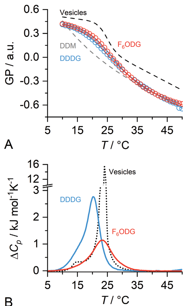
Figure 3. Gel-to-fluid phase transition of DMPC in DG nanodiscs by Laurdan fluorescence and DSC. A) Laurdan generalized polarization (GP) for hydrocarbon and fluorocarbon nanodiscs, DDM/DMPC mixed micelles, and unilamellar DMPC vesicles. DMPC (2 mM) in the form of unilamellar vesicles containing 0.5 mol% Laurdan was solubilized by addition of 5 mM DDM, 3 mM DDDG, or 3 mM F 6 ODG. B) Differential isobaric heat capacity, \Delta C_p , derived from DSC upscans for vesicles, hydrocarbon nanodiscs, and fluorocarbon nanodiscs. For nanodiscs, 4 mM DMPC in the form of vesicles was solubilized with 4 mM DDDG or F 6 ODG.
