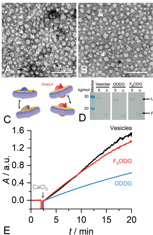
Figure 8. A,B) TEM images of DG nanodiscs made from A) 0.3 mM POPC, 1 μM OmpLA, and 1.0 mM DDDG or B) 0.25 mg ml -1 E. coli membrane and 0.2 mM F 6 ODG. White arrows exemplarily indicate face-on views of nanodiscs, and black arrows indicate edge-on views of nanodiscs. C) Schematic depiction of DG nanodiscs containing the membrane protein OmpLA or complex protein/lipid mixtures. D) SDS-PAGE of OmpLA-containing samples. Boiled (b) and unboiled (u) samples were loaded to assess the folding state of OmpLA in terms of folded (F) and unfolded (U) protein. E) Ca 2+ -induced enzyme activity measurements of OmpLA-containing vesicles, hydrocarbon nanodiscs, and fluorocarbon nanodiscs.
