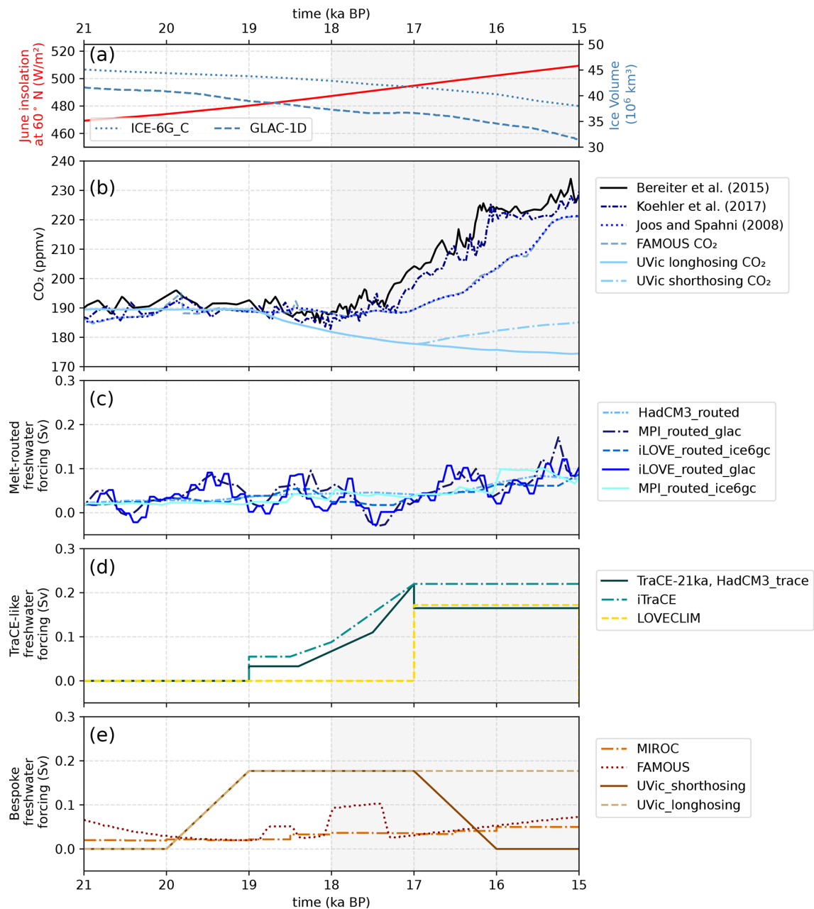
Figure 1. Climate forcings for the simulations. (a) Ice volume loss since the Last Glacial Maximum (LGM; 21 ka BP) as part of the ICE-6G_C ice sheet reconstruction (Argus et al., 2014; Peltier et al., 2015) and the GLAC-1D ice sheet reconstruction (Tarasov and Peltier, 2002; Tarasov et al., 2012; Briggs et al., 2014; Ivanovic et al., 2016) in light blue. June insolation at 60° N (Berger, 1978) is in red. (b) Atmospheric CO 2 concentrations are dependent on the simulation set-up. (c–e) Freshwater flux (Sv) for simulations with imposed meltwater. Melt-uniform simulations have the same total meltwater flux into the global ocean as melt-routed simulations (c), but in melt-uniform scenarios, the freshwater is spread through the entire ocean or across the whole ocean surface (see main text), rather than at point sources, and are hence so diluted or uniformly distributed as to have limited direct forcing power.
