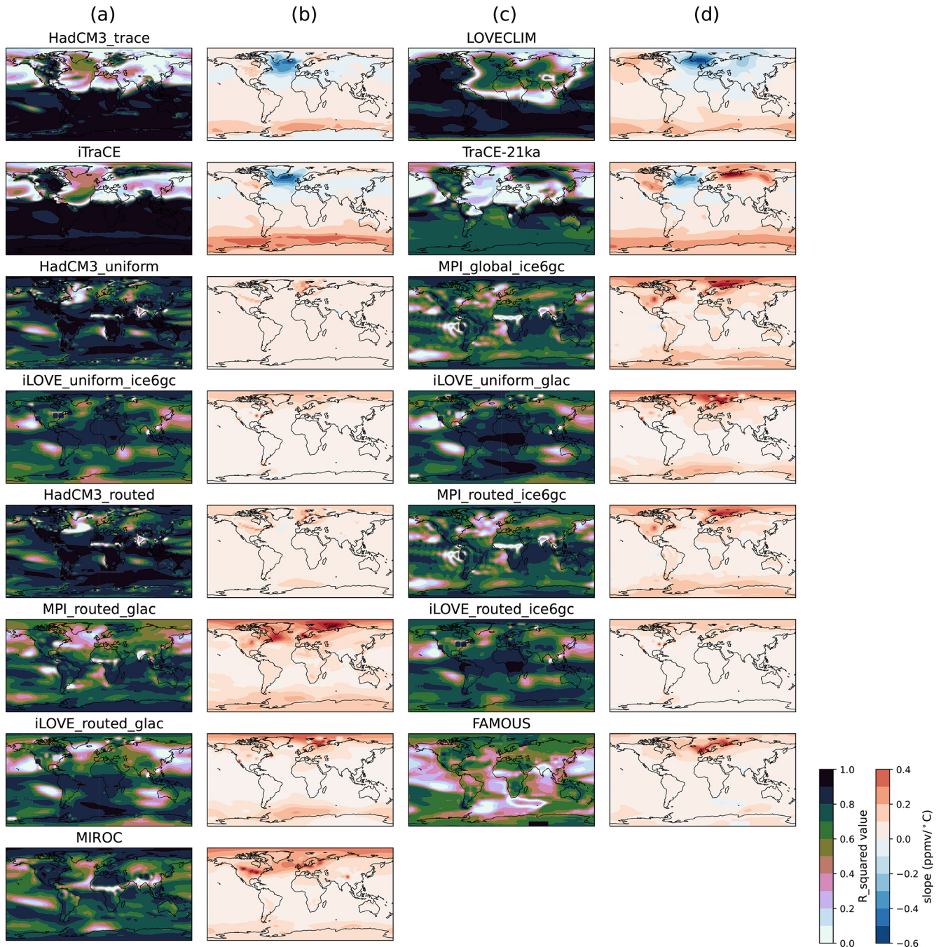
Figure 8. Spatial distribution of the temporal correlation of CO 2 concentration and surface air temperature using a linear regression model for the time period 20–15 ka BP using decadal means. Columns (a) and (c) show R^2 values as a result of the linear regression. Columns (b) and (d) show corresponding slopes to simulations in column (a) or (c) as a result of the linear regression.
