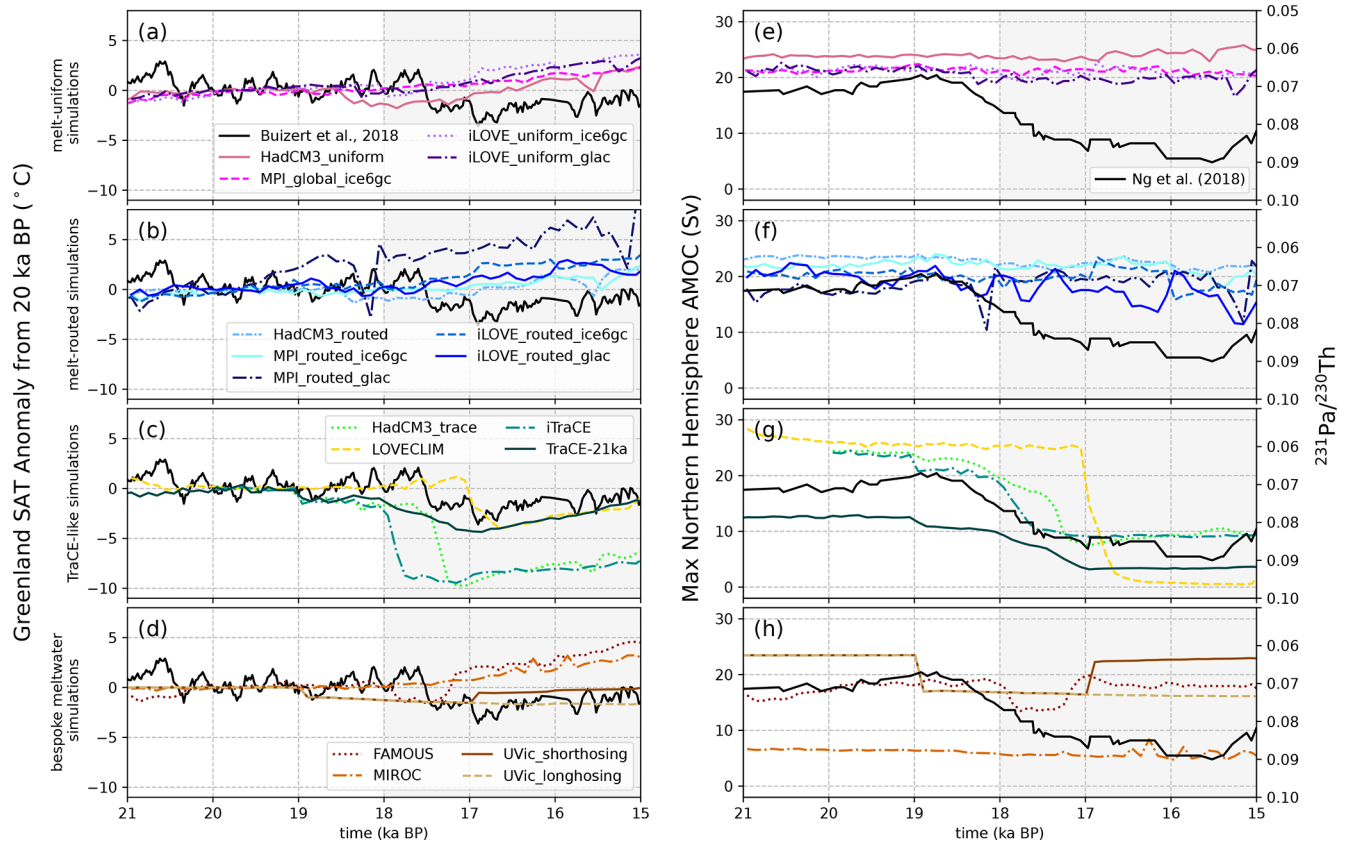
Figure 2. Centennial means for (a–d) Greenland (between 65 and 82°N and 30 and 55°W) surface air temperature anomaly from approximately the LGM (20–19.5 ka BP) for each simulation. (e–h) Maximum AMOC of the Northern Hemisphere at depth between 500 and 3500 m. For comparison, (a–d) includes Greenland surface air temperature proxy record from Buizert et al. (2018), plotted as an anomaly from 20 ka BP in black, and (e–h) includes the AMOC proxy ^{231}\text{Pa}/^{230}\text{Th} composite record published by Ng et al. (2018), plotted in black (note the arbitrary y-axis scaling). The grey-shaded region denotes the timing of Heinrich Stadial 1.
