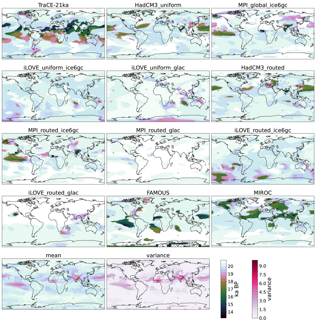
Figure 5. Year of first significant warming from 20 ka BP, where “significant warming” is determined as discussed in Sect. 3. Hatching denotes where significant warming did not occur before 13 ka BP.
