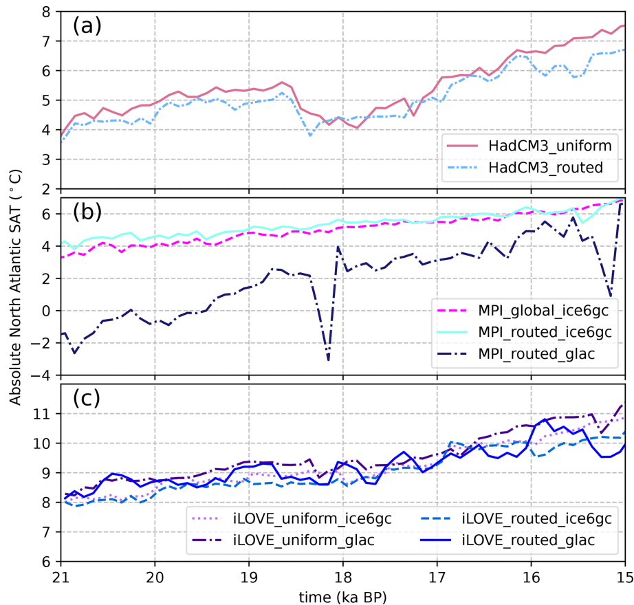
Figure 9. Absolute surface air temperature in the North Atlantic (between 35 and 60° N and –60 and 0° E) for the HadCM3, MPI-ESM, and iLOVECLIM simulations. Note that to capture variability, the y-axis limits are not the same for each panel. Absolute surface air temperature in the North Atlantic for the entire ensemble is shown in Fig. S5e–h.
