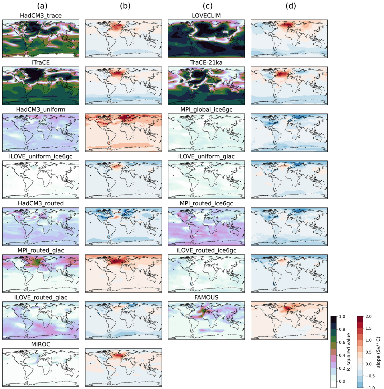
Figure 7. Spatial distribution of the temporal correlation of AMOC strength and surface air temperature using a linear regression model for the time period 20–15 ka BP using decadal means. Columns (a) and (c) show R^2 values as a result of the linear regression. Columns (b) and (d) show corresponding slopes to simulations in column (a) or (c) as a result of the linear regression.
