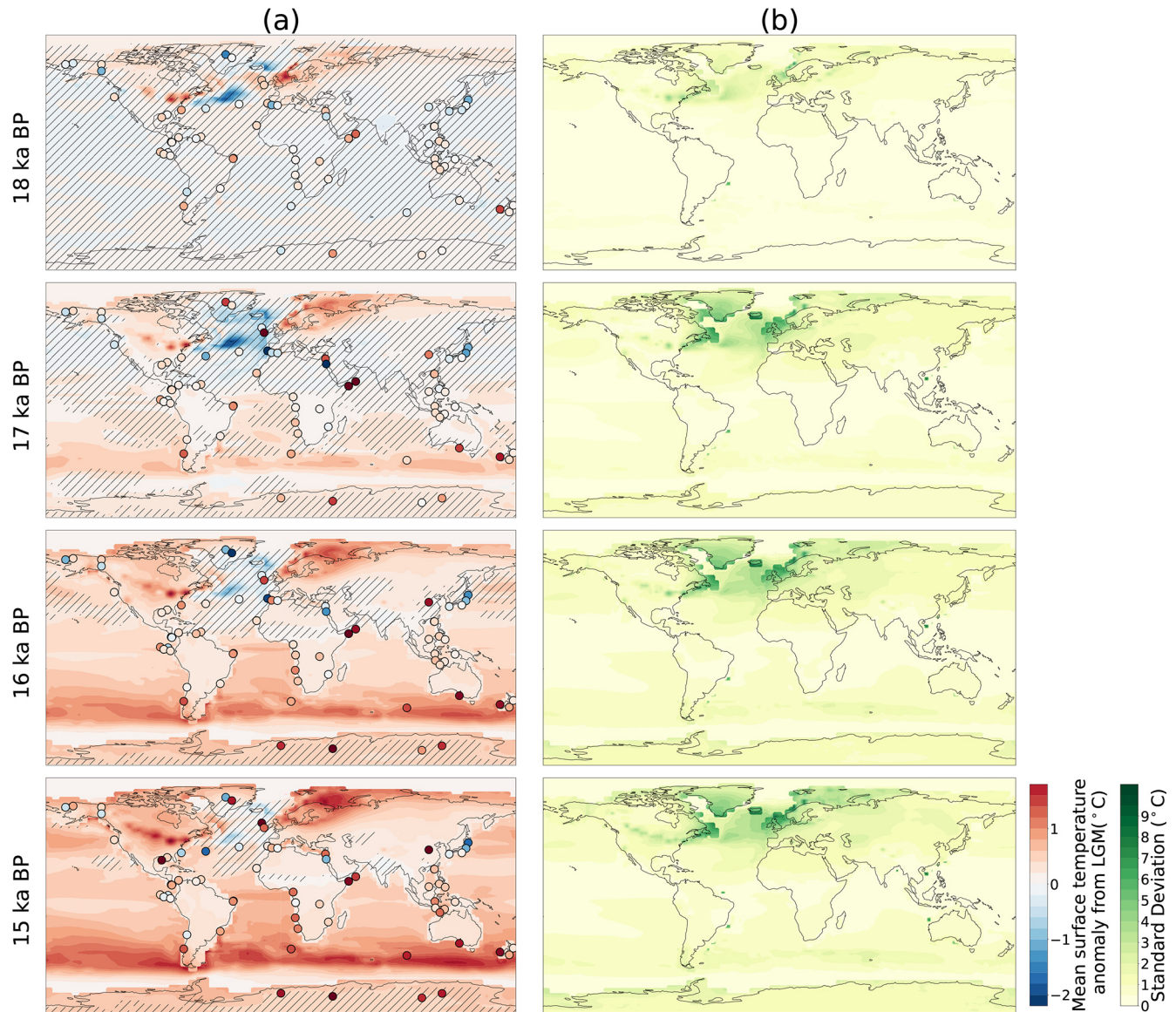
Figure 4. (a) Multi-model mean of decadal surface temperature anomaly from the LGM (20–19.5 ka BP) at each time step labelled (not including the UVic simulations). Hatching denotes areas in which less than 70 % of the simulations agree with the sign of the mean. The agreement with the sign of the mean was determined using a one sample t test at 95 % confidence by testing if the simulation and the mean were both significantly different from zero in the same direction. Column (b) is the same as column (a) but showing the variance. Filled circles show the proxy surface temperature stack from Shakun et al. (2012) on the same colour scale; 18, 17, 16, and 15 ka BP are calculated as 60-year decadal means centred around the respective time period (e.g. from 17.97 to 18.03 ka BP for 18 ka BP).
