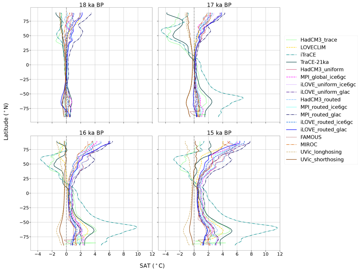
Figure 3. Zonal average of decadal mean surface air temperature as anomalies from the LGM (20–19.5 ka BP) for each simulation; 18, 17, 16, and 15 ka BP are calculated as 60-year decadal means centred around the respective time period (e.g. from 17.97 to 18.03 ka BP for 18 ka BP).
