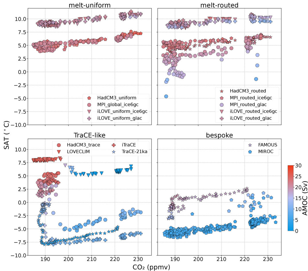
Figure 6. Absolute surface air temperature over the North Atlantic (between 35 and 60°N and –60 and 0°E) as a function of CO 2 concentration with symbol shading representing the strength of the AMOC (Sv) split into groups defined by meltwater scenario. The 50-year means are shown for each simulation except for MIROC, for which decadal means are shown to capture its temporally finer-scale variability. See Fig. S6 for the same analysis displayed as anomalies from 20 ka BP.
