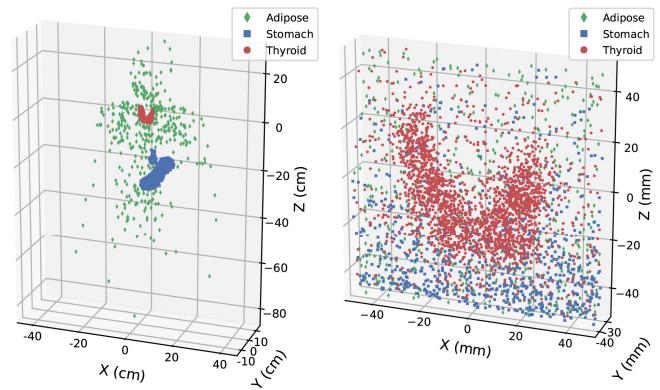
Fig. 17. Left: Emission positions of gamma-rays detected by the camera. Right: Positions of interaction of gamma-rays in the scintillator. Each event is classified according to its region of origin (adipose tissue, stomach, and thyroid). It corresponds to the weakest simulated shielding configuration, WH-2 WTS-0 PbT-2.
