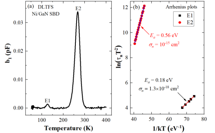
Figure 12. (a) Measured DLTFs for Ni/GaN SBD (first order Fourier sine coefficient b_1 used). (b) Arrhenius plots for traps E1 and E2.
