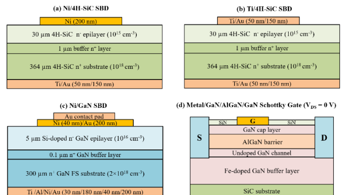
Figure 1. Schematic cross-section for (a) Ni/4H-SiC SBD, (b) Ti/4H-SiC SBD, (c) Ni/GaN SBD, and (d) GaN/AlGaIn/GaN HEMT.
