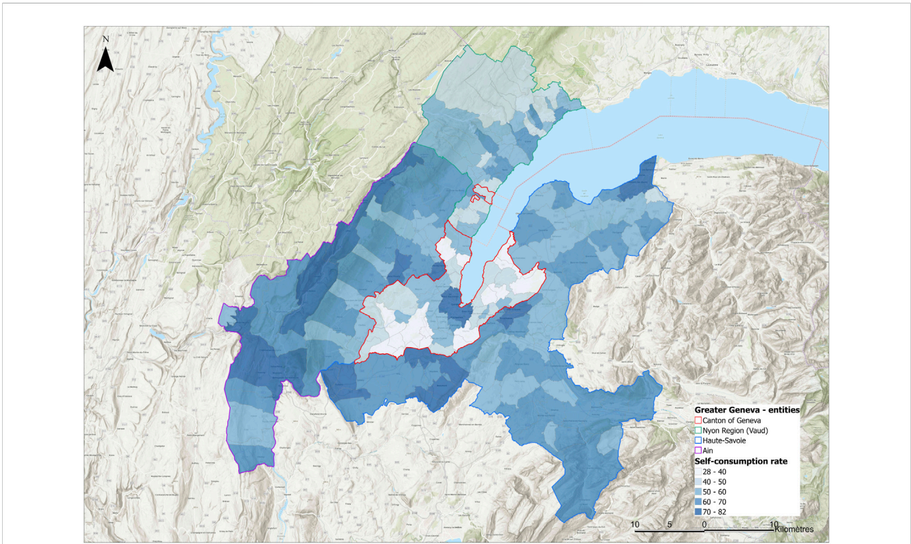
FIGURE 12 Global statistics by the commune in the Greater Geneva, indicating the potential self-consumption ratio by photovoltaic panels.
