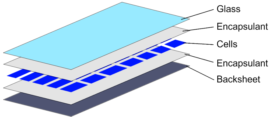
Figure 1. The main five layers of PV modules (adapted from [4]).
