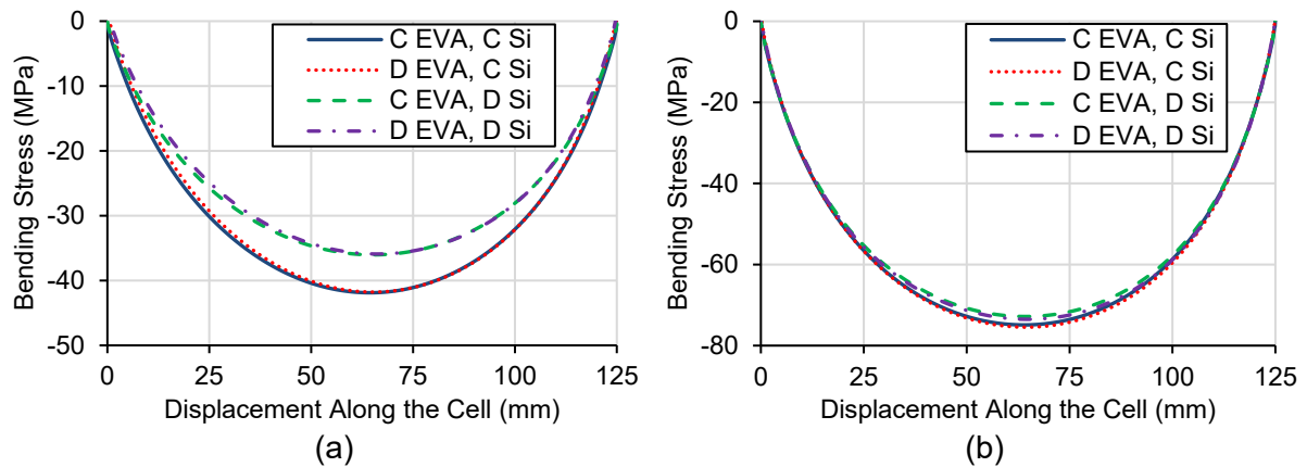
Figure 9. Numerical predictions of different CTE models of the cell stress: (a) at 22°C, and (b) at -35°C.
