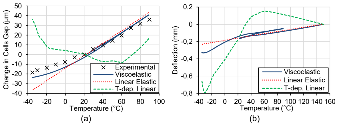
Figure 6. Numerical predictions of different EVA models: (a) change in cells gap, and (b) module deflection (experimental data taken from [9]).
