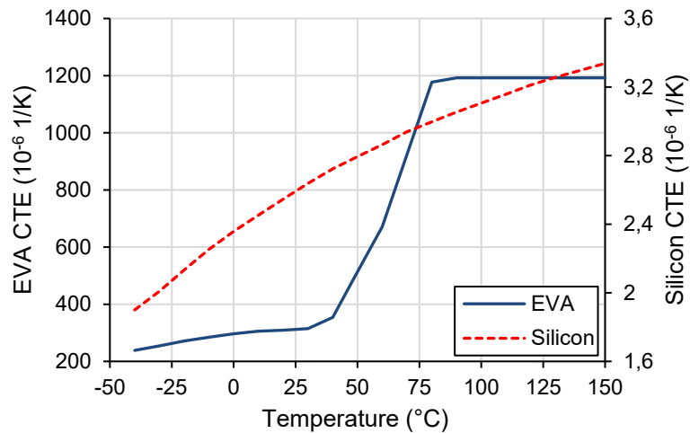
Figure 4. Temperature-dependent CTE curves of silicon and EVA [8], [10], [11].
