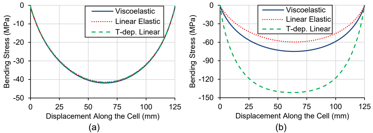
Figure 7. Numerical predictions of different EVA models of the cell stress: (a) at 22°C, and (b) at -35°C.
