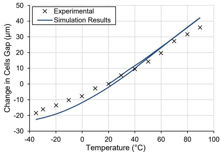
Figure 5. The numerical predictions of the change in cells gap using the reference material models. (Experimental data taken from [9]).
