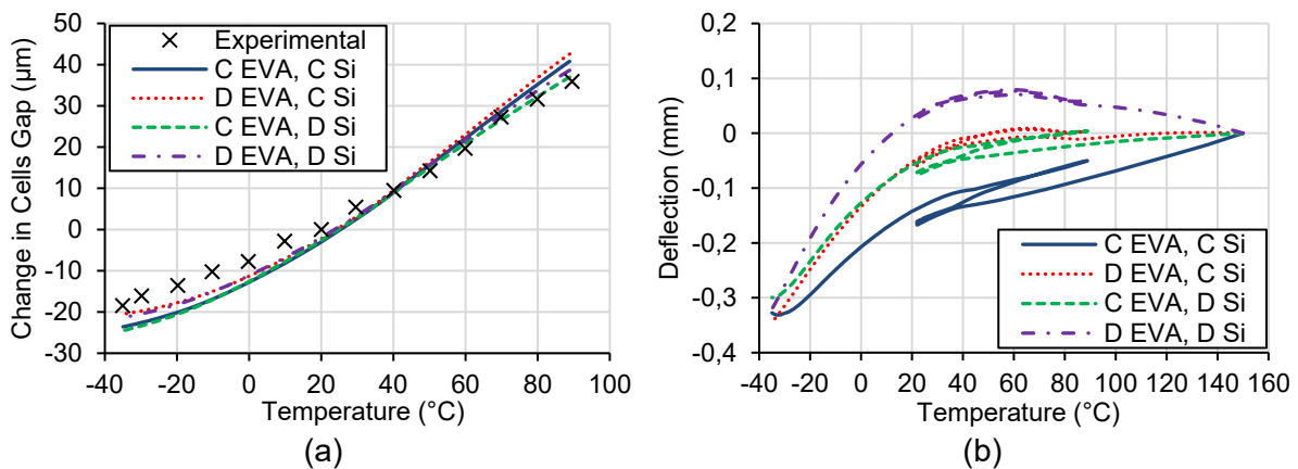
Figure 8. Numerical predictions of different CTE models of EVA and silicon: (a) change in cells gap, and (b) module deflection (Experimental data taken from [9]).
