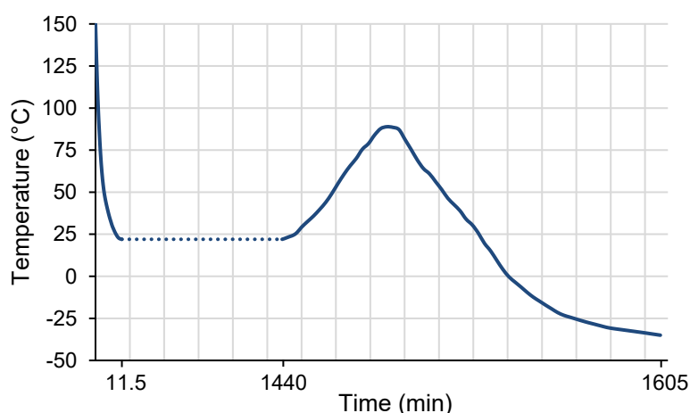
Figure 3. Temperature profile of the cells gap experiment as a function of time [9].
