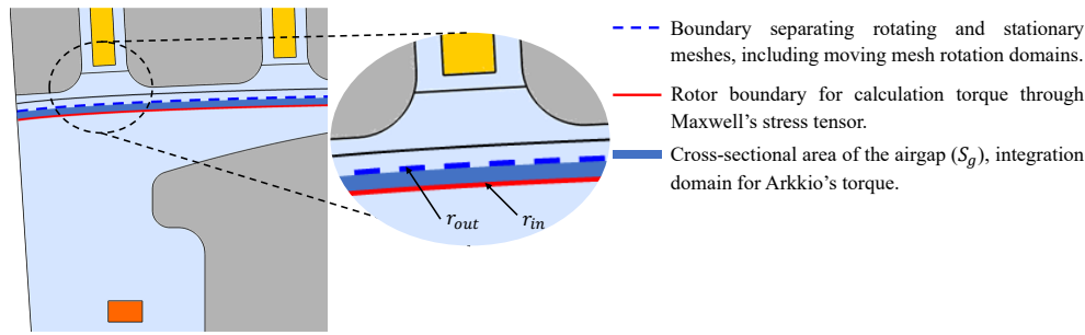
Figure 4. Schematic drawing defining the boundaries between the stator and the rotor. The air-gap region is divided in sub-regions. There, the blue line separating the rotating mesh from the static mesh does not coincide with the red line over which the torque is computed. This setting allows refining the mesh to compute the torque with greater accuracy independently of the moving interface for which the mesh finesse can be reduced.
