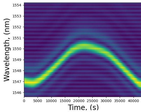
Figure 1. GAVgram representing the variation of the Bragg wavelength of an FBG subjected to temperature variations.
