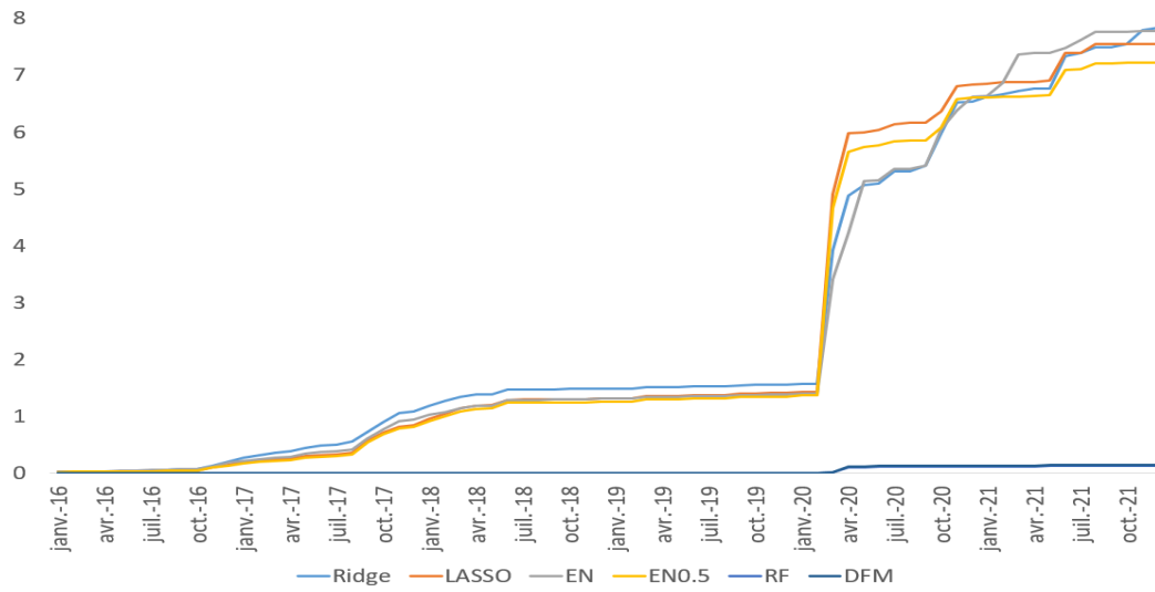
Figure 3: Cumulative squared prediction errors during the full out-of-sample period – 2016M1-2021M12 – with the regional database.
