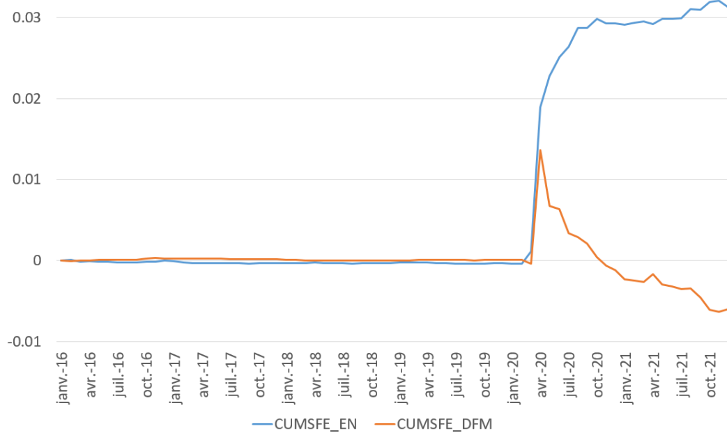
Figure 4: Cumulative sum of squared forecast error (CUMSFE) from the regional and large databases.
