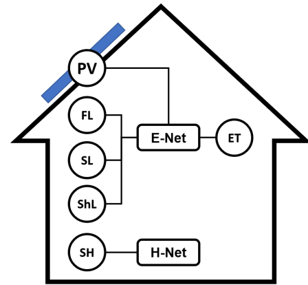
Figure 5: A conceptual implementation structure of the optimisation component (ABO) at an individual building level - Linking different electrical loads included fixed loads (FL), Shiftable loads (SL), Sheddable loads (ShL), and PV at an electrical Net agent (E-Net) with a connection to the External Tie (ET), while space heating (SH) linked to heating Net agent (H-Net)
