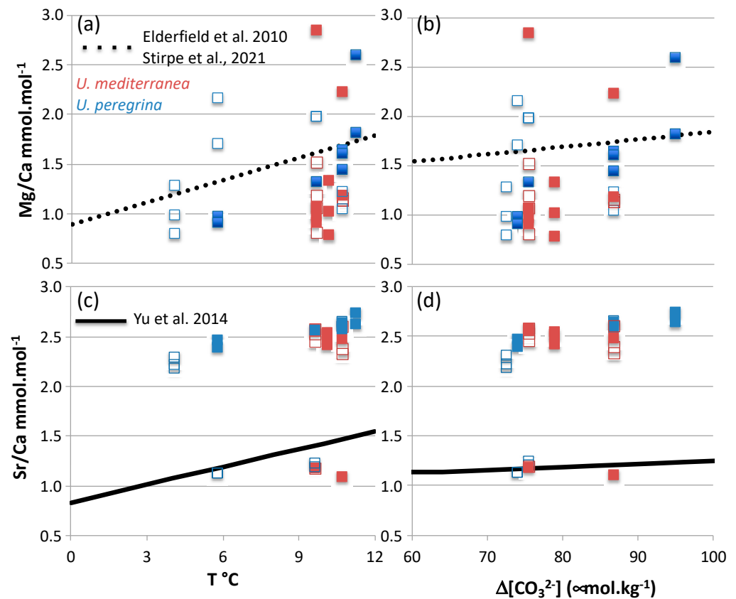
Figure 4. Variations in Mg/Ca (a,b) and Sr/Ca (c,d) versus temperature (a,c) and \Delta[\text{CO}_3^{2-}] (b,d) for Uvigerina peregrina (blue) and Uvigerina mediterranea (red). Empty and full symbols represent data obtained from dead and live specimens, respectively. The black curves were obtained on Uvigerina spp. by [51] (solid line) and [29,31], the two latest calibrations being statistically indistinguishable for temperature (dashed line).
