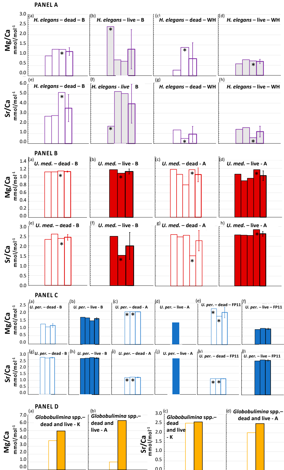
Figure 6. Comparison between results from dead and live specimens (empty and full bar, respectively). The average values are reported as the last bar with bold contour, error is given as 1\sigma . Asterisks indicate results obtained by ICP-MS, the other data being measured by ICP-OES. [Panel A: Purple:
