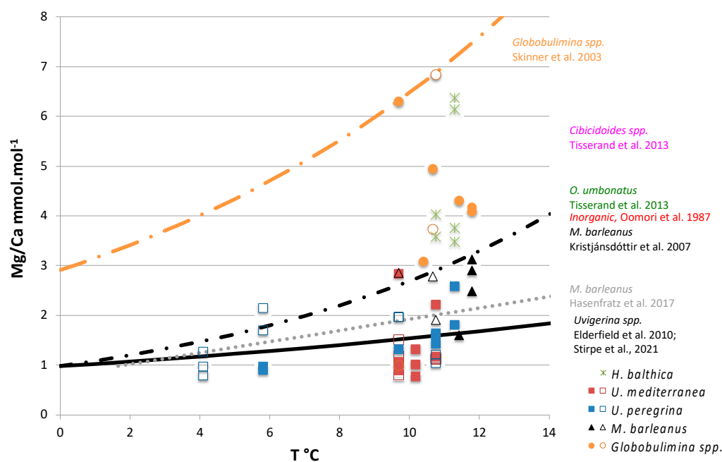
Figure 8. Compilation of published data on the relationship between Mg/Ca and temperature for the studied calcitic species and other species: orange line and circles: Globobulimina spp. [71]; pink line: Cibicidoides spp. and green line: Oridorsalis umbonatus [32]; Melonis barleeanum : black dotted line and triangles [69] and grey dotted line [70]; Uvigerina spp.: red and blue squares, and bold black line [29,31]. The calibration obtained by precipitation of inorganic calcite is also reported in light red [7]. Empty and full symbols represent data obtained from dead and live specimens, respectively.
