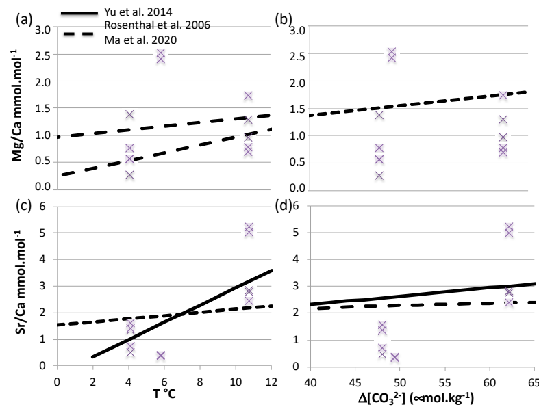
Figure 3. Variations in Mg/Ca (a,b) and Sr/Ca (c,d) versus temperature (a,c) and \Delta[\text{CO}_3^{2-}] (b,d) for Hoeglundina elegans . Empty and solid symbols (crosses) represent data obtained on dead and live specimens, respectively. The black curves were obtained on the same species by [51] (solid line) and [50,67] (dotted line).
