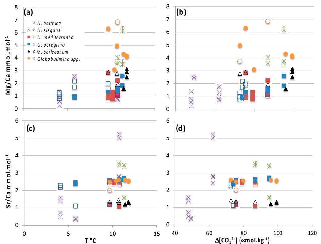
Figure 2. Variations in Mg/Ca (a,b) and Sr/Ca (c,d) versus temperature (a,c) and \Delta[\text{CO}_3^{2-}] (b,d). Empty and full symbols represent data obtained from dead and live specimens, respectively. Green crosses: Hyalinea balthica ; purple squares and crosses: Hoeglundina elegans ; red squares: Uvigerina mediterranea ; blue squares: Uvigerina peregrina ; black triangles: Melonis barleeanum ; orange circles: Globobulimina spp.
