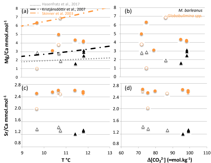
Figure 5. Variations in Mg/Ca (a,b) and Sr/Ca (c,d) versus temperature (a,c) and \Delta[\text{CO}_3^{2-}] (b,d) for Melonis barleeanum (black) and Globobulimina spp. (orange). Empty and solid symbols represent data obtained from dead and live specimens respectively. The dotted black and grey curves were obtained on Melonis barleeanum by [69,70], respectively, and the orange curve on Globobulimina affinis by [71].
