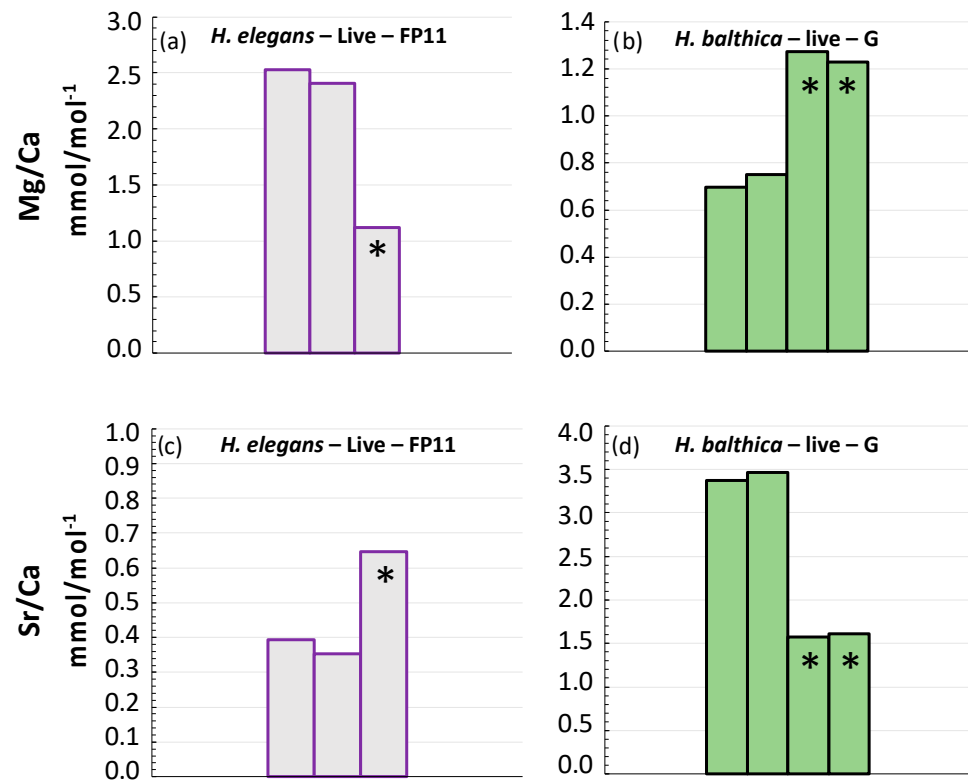
Figure 7. Comparison between results of living specimens from the same station measured by ICP-OES and ICP-MS (asterisks). (a,c) Purple: living Hoeglundina elegans from station FP11; (a) Mg/Ca; (c) Sr/Ca. (b,d) Green: living Hyaline balthica from station G; (b) Mg/Ca; (d) Sr/Ca.
