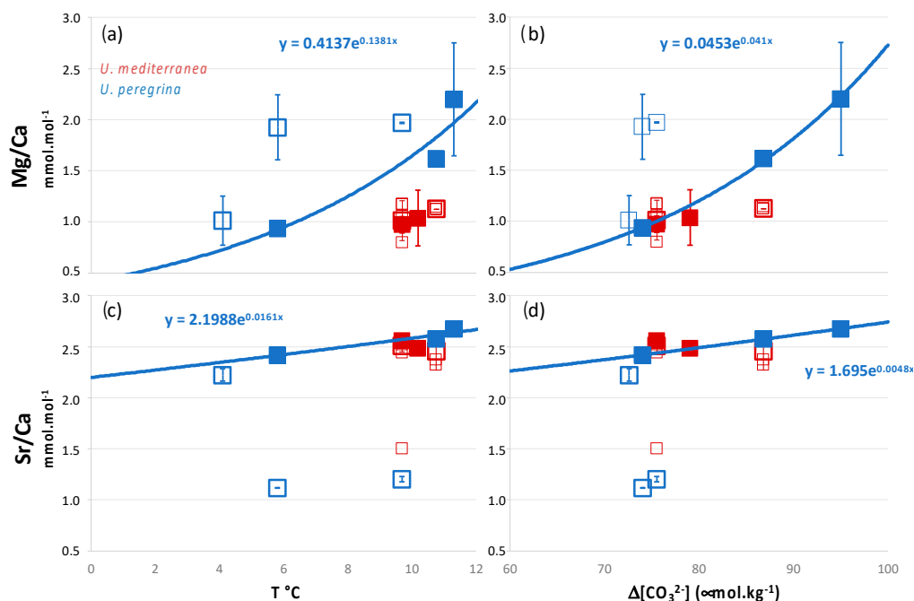
Figure 9. Variations in Mg/Ca (a,b) and Sr/Ca (c,d) versus temperature (a,c) and \Delta[\text{CO}_3^{2-}] (b,d) for Uvigerina peregrina (blue) and Uvigerina mediterranea (red). Empty and full symbols represent data obtained from dead and live specimens, respectively. The average values are indicated with larger symbols with error bars corresponding to the external reproducibility (Table 4). The blue curve corresponds to the calculated correlation including only the data measured in living specimens of U. peregrina (see text for explanation).
