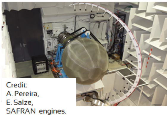
Figure 6. Photo of the “Phare 2” facility.
