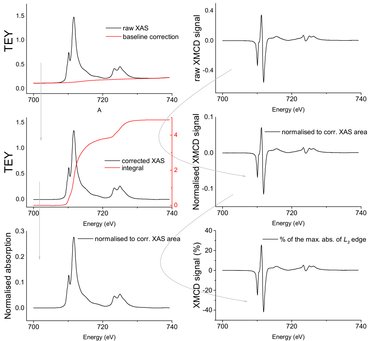
Figure S14. Graphical representation of the different steps for the normalization of the Fe L_{2,3} edges XAS spectra and XMCD signals in \gamma\text{-Fe}_2\text{O}_3 , \gamma\text{-Fe}_2\text{O}_3\{\text{Co}(\text{TPMA})\} and \gamma\text{-Fe}_2\text{O}_3\{\text{Ni}(\text{TPMA})\} .
