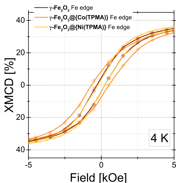
Figure 3. Field-dependence of the Oh Fe L_3 edge XMCD signals for \gamma\text{-Fe}_2\text{O}_3 , \gamma\text{-Fe}_2\text{O}_3\text{@[Co(TPMA)]} and \gamma\text{-Fe}_2\text{O}_3\text{@[Ni(TPMA)]} at 4 K.
