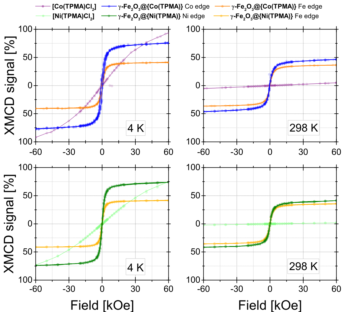
Figure 4. Field-dependence of the Oh Fe, Co and Ni L_3 edge XMCD signals for \gamma\text{-Fe}_2\text{O}_3@[\text{Co}(\text{TPMA})] , \gamma\text{-Fe}_2\text{O}_3@[\text{Ni}(\text{TPMA})] , [\text{Co}(\text{TPMA})\text{Cl}_2] and [\text{Ni}(\text{TPMA})\text{Cl}_2] at 4 K and 298 K.
