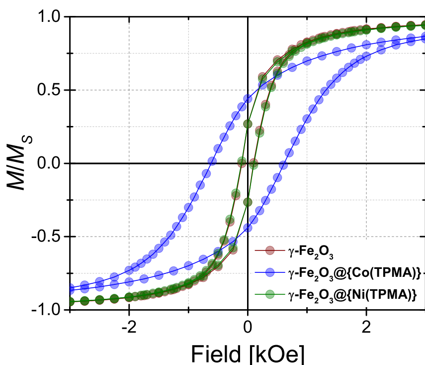
Figure 1. Magnetization v. field measurements for \gamma\text{-Fe}_2\text{O}_3 , \gamma\text{-Fe}_2\text{O}_3@{\text{Co}(\text{TPMA})} and \gamma\text{-Fe}_2\text{O}_3@{\text{Ni}(\text{TPMA})} at 5 K. Saturation values have been normalized to 1 at 50 kOe.
