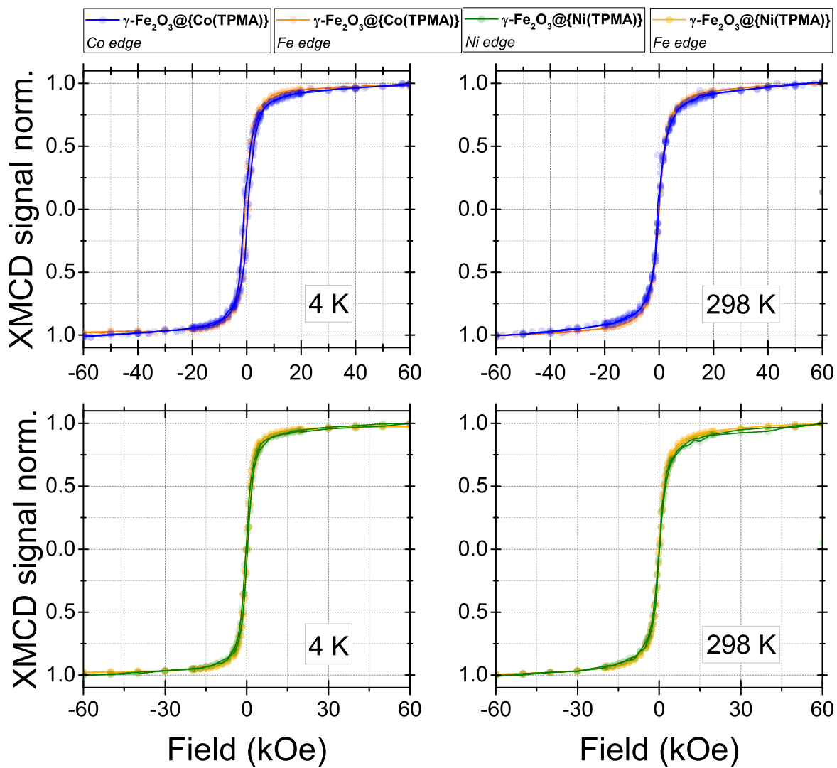
Figure S19. Field-dependence of the Oh Fe L_3 , Co L_3 and Ni L_3 edges normalized XMCD signals for \gamma\text{-Fe}_2\text{O}_3@\{\text{Co}(\text{TPMA})\} and \gamma\text{-Fe}_2\text{O}_3@\{\text{Ni}(\text{TPMA})\} at 4 K and 298 K.
