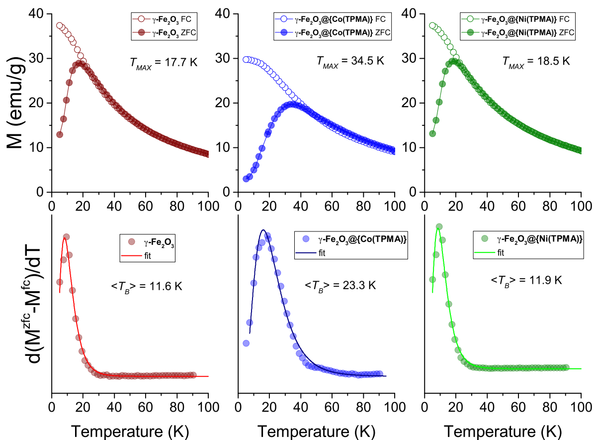
Figure S8. ZFC/FC curves measured by SQUID at 50 Oe between 5 and 100 K, with T_{MAX} values and fitting of \langle T_B \rangle values for compounds \gamma\text{-Fe}_2\text{O}_3 , \gamma\text{-Fe}_2\text{O}_3@{\text{Co(TPMA)}} and \gamma\text{-Fe}_2\text{O}_3@{\text{Ni(TPMA)}} .
