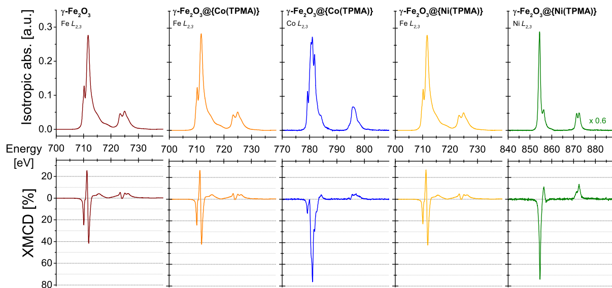
Figure 2. XAS spectra and XMCD signals at the Fe, Co and Ni L_{2,3} edges measured at 4 K and \pm 60 kOe for compounds \gamma\text{-Fe}_2\text{O}_3 , \gamma\text{-Fe}_2\text{O}_3@{\text{Co(TPMA)}} and \gamma\text{-Fe}_2\text{O}_3@{\text{Ni(TPMA)}} . The XMCD signal is plotted as the percentage of the maximum intensity in the XAS spectrum.
