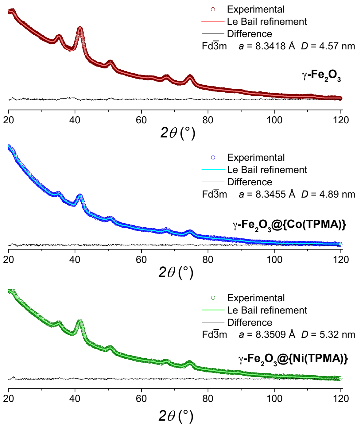
Figure S5. Powder X-ray diffraction patterns, Le Bail fit results and size determinations for compounds \gamma\text{-Fe}_2\text{O}_3 , \gamma\text{-Fe}_2\text{O}_3@{\text{Co(TPMA)}} and \gamma\text{-Fe}_2\text{O}_3@{\text{Ni(TPMA)}} .
