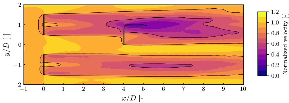
FIGURE 13 2D map of the normalized velocity ( u_x/u^\infty ) of the numerical 'TI 2' case.
