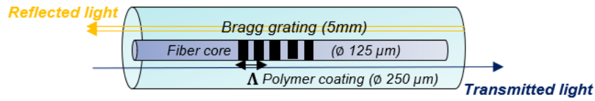
Figure 3: Complete structure of the FBG sensor and its principal function.
