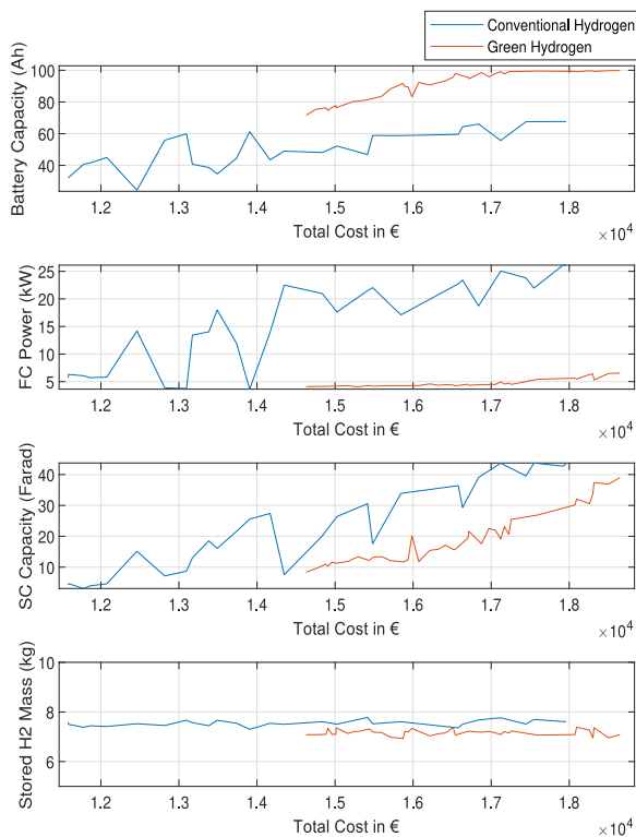
Fig. 15. Sizing result for the PFCVEs: Conventional hydrogen vs. Green hydrogen.
