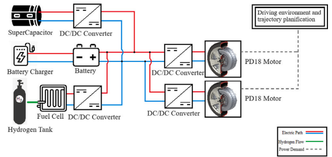
Fig. 1. Powertrain architecture.
