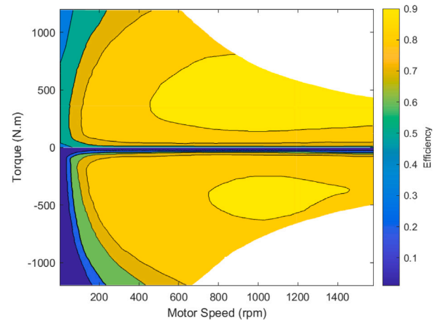
Fig. 2. Motor efficiency and torque bounds; Positive torque during motoring, negative torque during braking.
