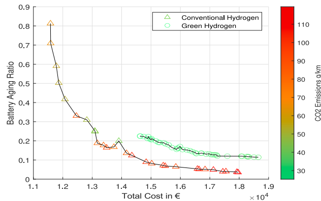
Fig. 14. Comparative Pareto Fronts for PFCEVs: Conventional hydrogen vs. Green hydrogen.
