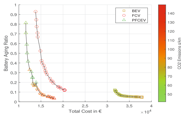
Fig. 13. Comparative Pareto Fronts for PFCEV, FCV and BEV.
