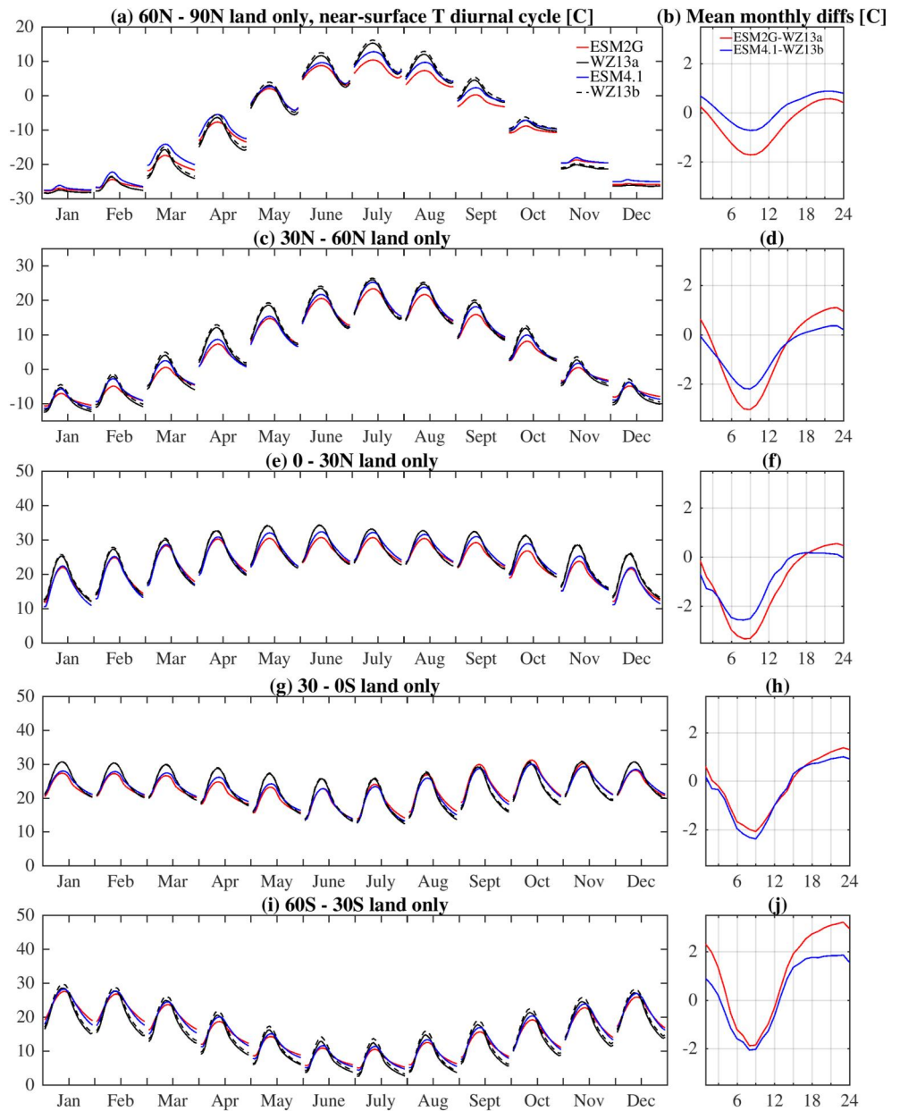
Figure 5. Left column: Monthly mean diurnal cycles averaged over land areas in zonal bands of 30° latitude each from ESM2G (red), ESM4.1 (blue), and the WZ13 observation-based data product of A. Wang and Zeng (2013) (WZ13a for years matching ESM2G, WZ13b for years matching ESM4.1; see Figure 4 caption for details). Right column: Corresponding annual mean differences in diurnal cycles, model—observations (ESM2G—WZ13a in red; ESM4.1—WZ13b in blue). The horizontal axis is the local time of day.
