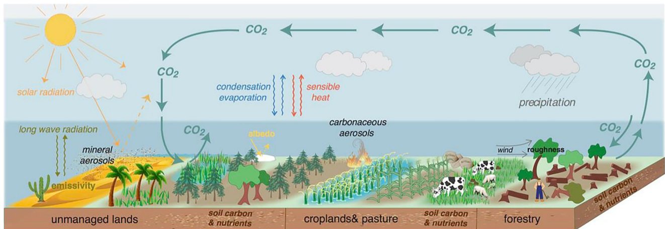
Figure 1. Schematic of land surface processes (e.g., dynamic vegetation competition, land use) and land-atmosphere interactions including radiative, hydrological, CO 2 , and dust fluxes in Geophysical Fluid Dynamics Laboratory LM4.1 land model.
