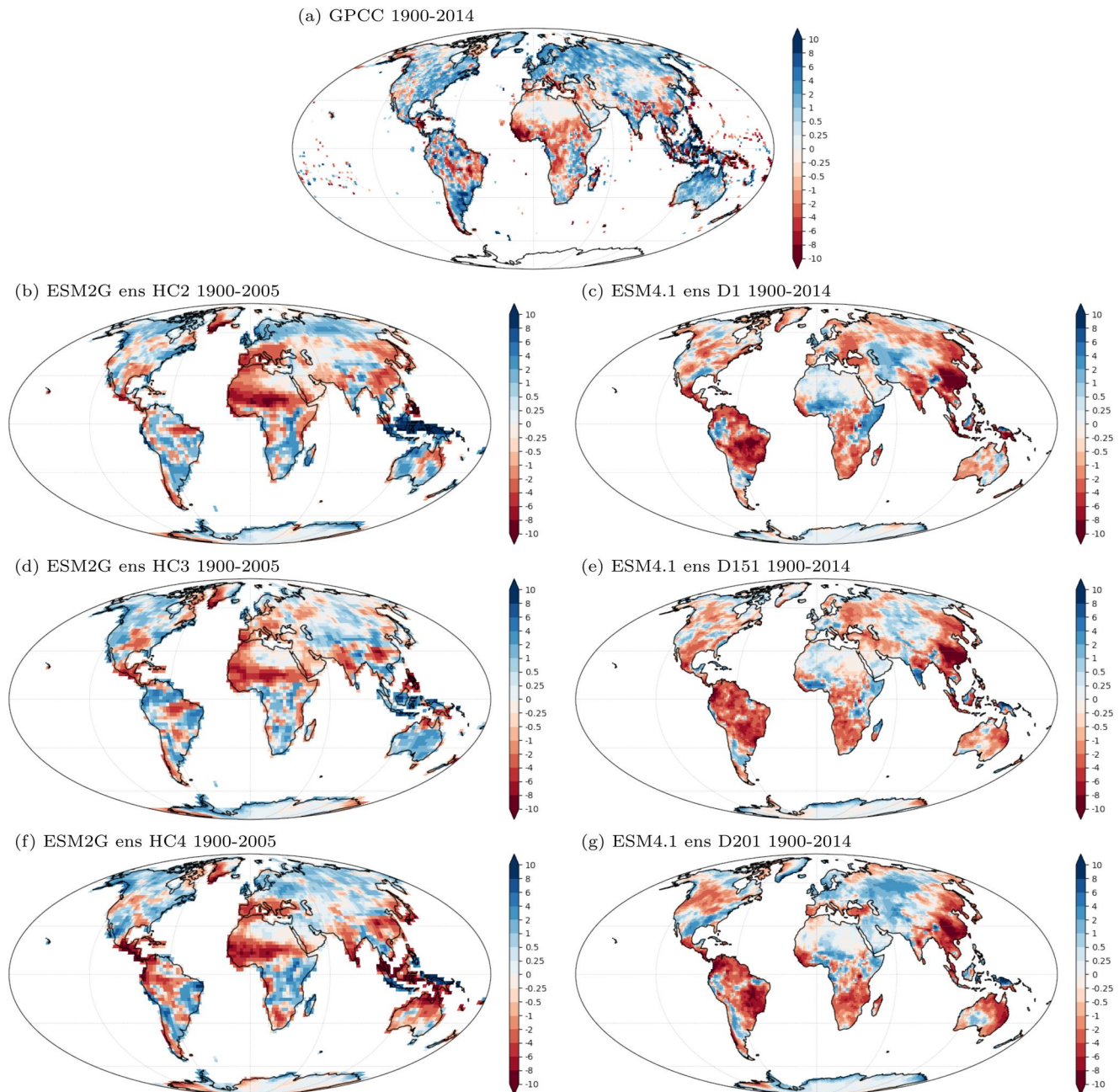
Figure 13. Observed (GPCCC data over land) and simulated precipitation trends for long-term historical climate since 1900, mm/year/decade. Panels (b, d, and f) show three ensemble members of ESM2G simulation, and panels (c, e, and g)—show three ensemble members of ESM4.1. Grid cells with sparse observations in the GPCCC time series are not masked out.
