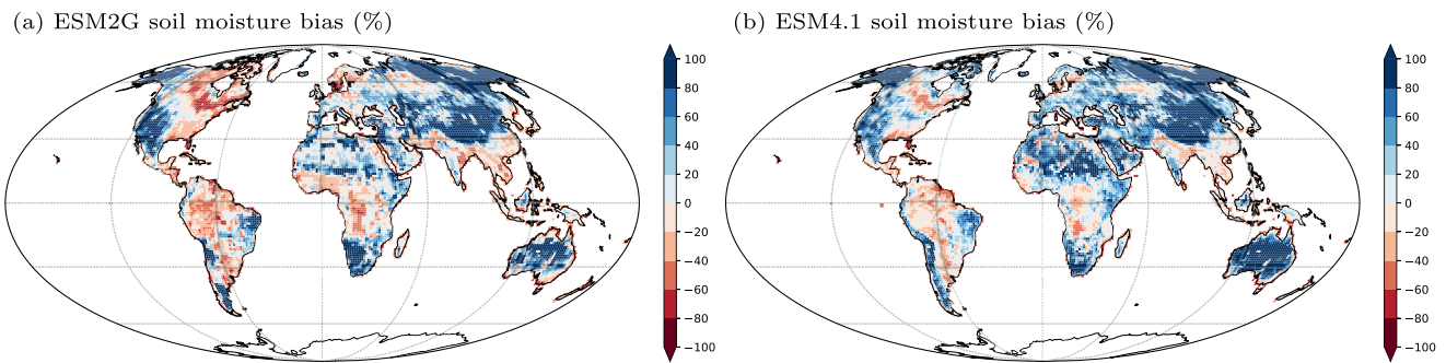
Figure 9. Bias (%) in ESM2G and ESM4.1 annual-mean soil moisture relative to observational estimates from the SMAP mission (L3 v6 product). SMAP data spans the period 2015–2019 and is representative of the top 0–5 cm soil layer (Das et al., 2019; P. E. O’Neill et al., 2019), and model outputs were averaged over the same period and depth. Both ESM2G output and SMAP data were regridded to the ESM4.1 grid.
