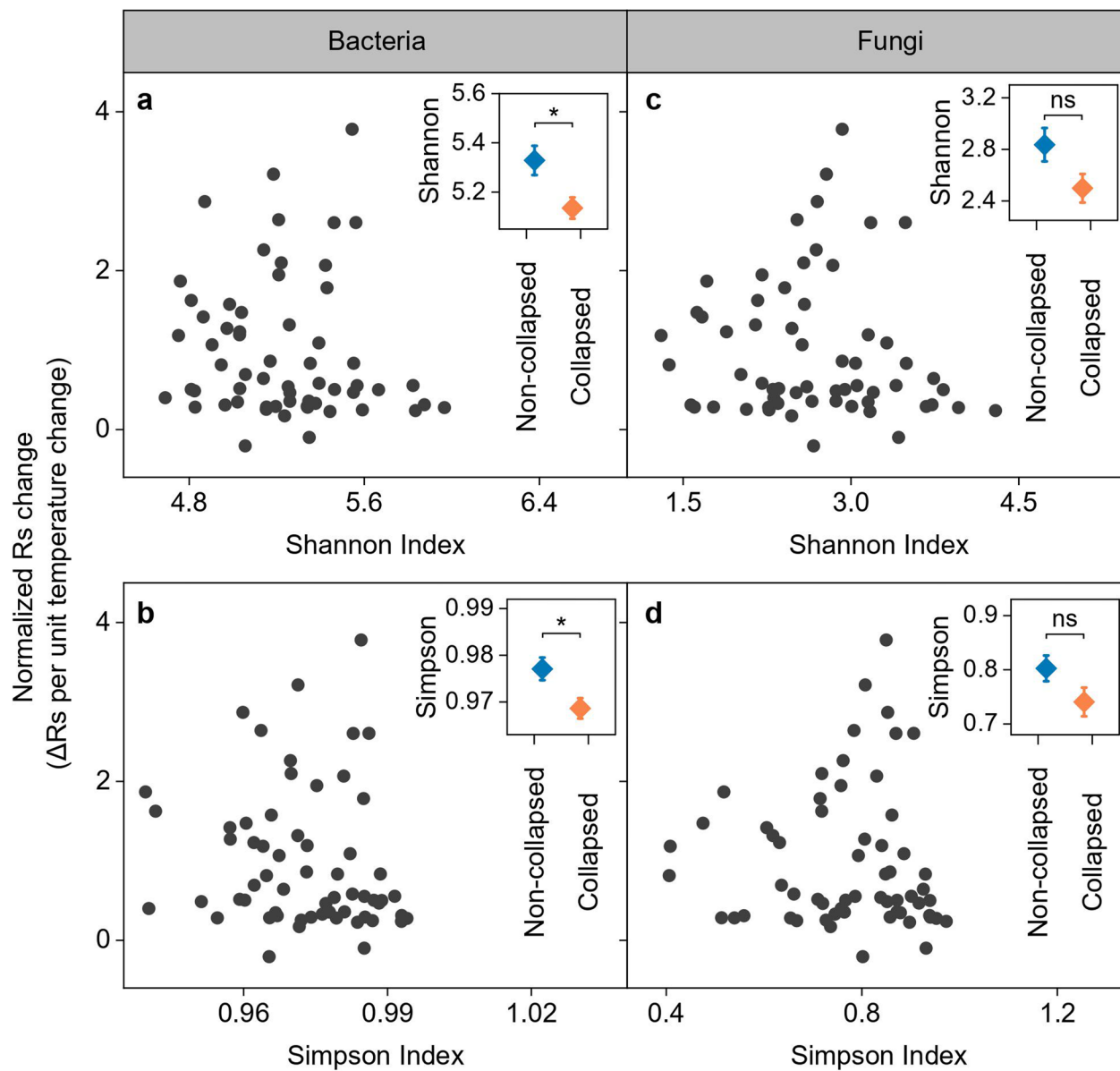
Extended Data Fig. 9 | Thermokarst-induced differences in topsoil (0–10 cm) microbial diversity and their relationships with the normalized soil respiration (Rs) change at the Shaliuhe site. a–d, Relationships of normalized Rs change with Shannon and Simpson indices for bacterial (a, b) and fungal (c, d) communities. The inserts denote differences in Shannon and
