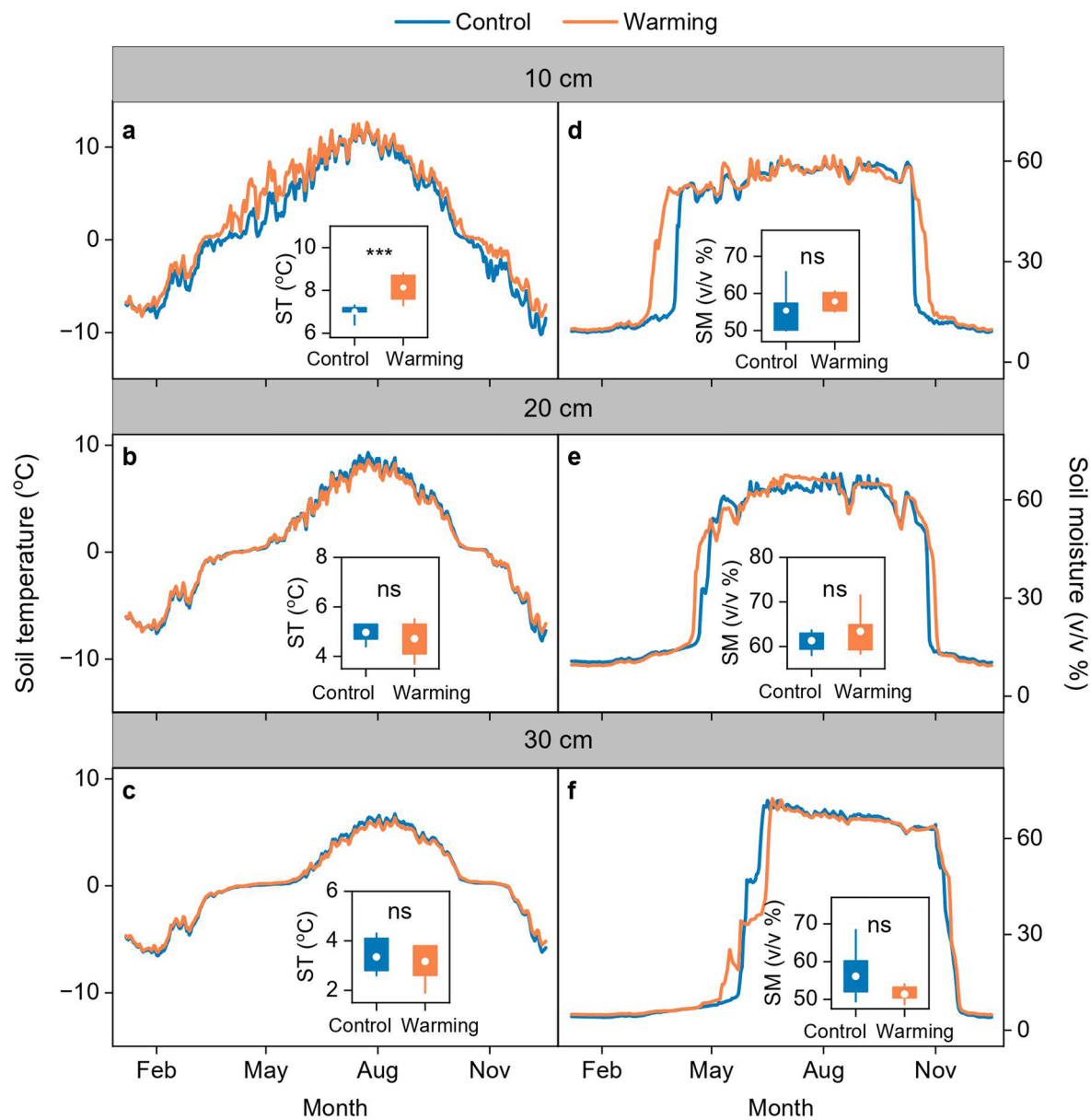
Extended Data Fig. 5 | Effects of experimental warming on temperature and moisture in different soil layers of non-collapsed areas at the Shaliuhe site. a-c, Daily soil temperature at depth of 10 cm (a), 20 cm (b) and 30 cm (c) from January to December. d-f, Daily soil moisture at depth of 10 cm (d), 20 cm (e) and 30 cm (f) from January to December. The inserts show the averages of soil temperature and moisture across the growing season (May - October).
