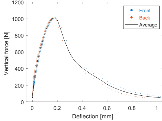
Figure 13: Vertical force as a function of the deflection (which is significantly different from the actuator displacement, see Figure 10(b)) calculated on the front and back surfaces, as well as the average among them, for the three-point bend test.
