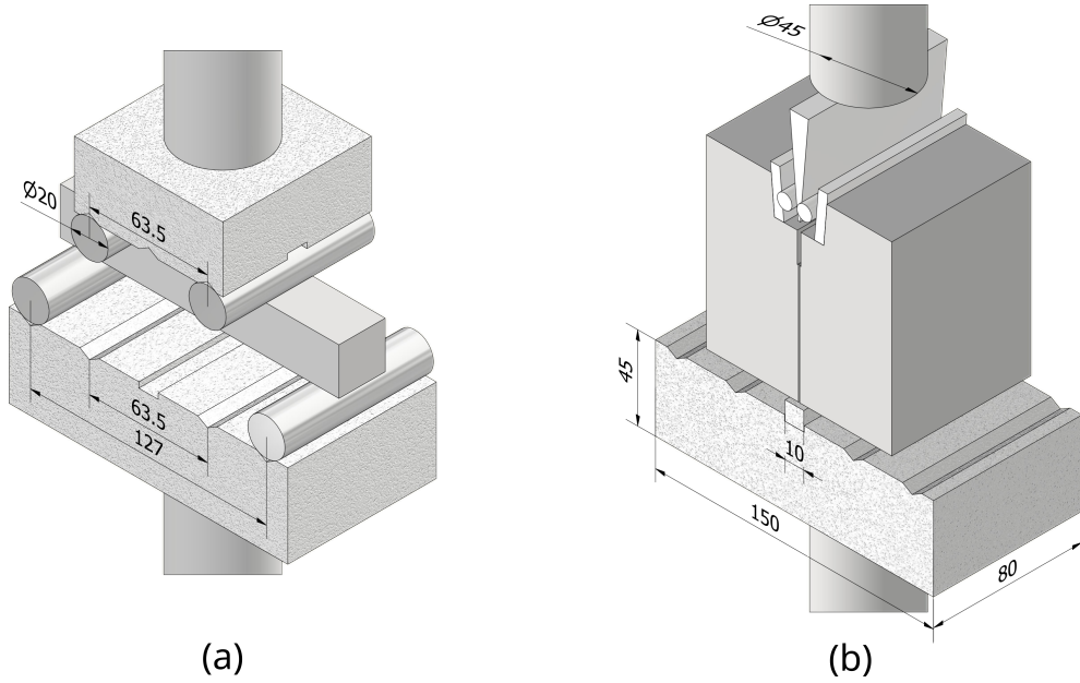
Figure 5: 900°C setups for (a) bend experiments and (b) WSTs. Dimensions are given in mm.
