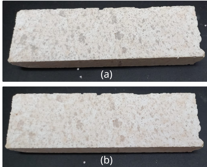
Figure 7: Silicon carbide slurry pattern of a parallelepipedic sample (of approximately 10 \times 25 \times 120 \text{ mm}^3 ) made of the same material used in three-point bending (Section 3.2) and WST (Section 3.3) (a) before and (b) after being heated up to 900^\circ\text{C} .
