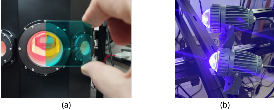
Figure 6: (a) Effect of the blue bandpass filter on image acquisition at 900°C. (b) 10W blue LED illumination dedicated to one of the furnace windows.
