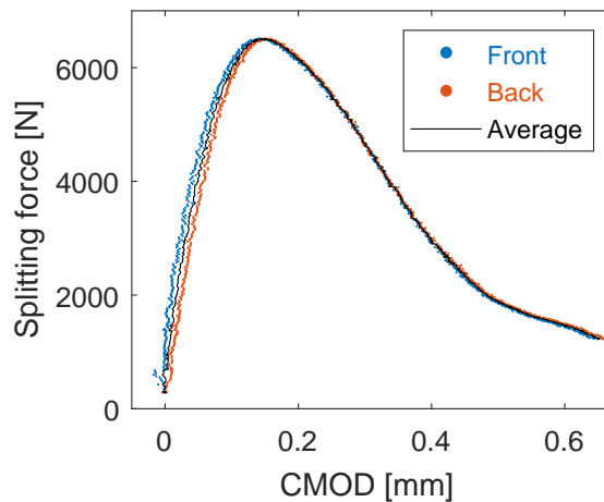
Figure 17: Horizontal loading curves for the Wedge Splitting Test (WST) performed at 900°C with the CMODs measured for both opposite surfaces.
