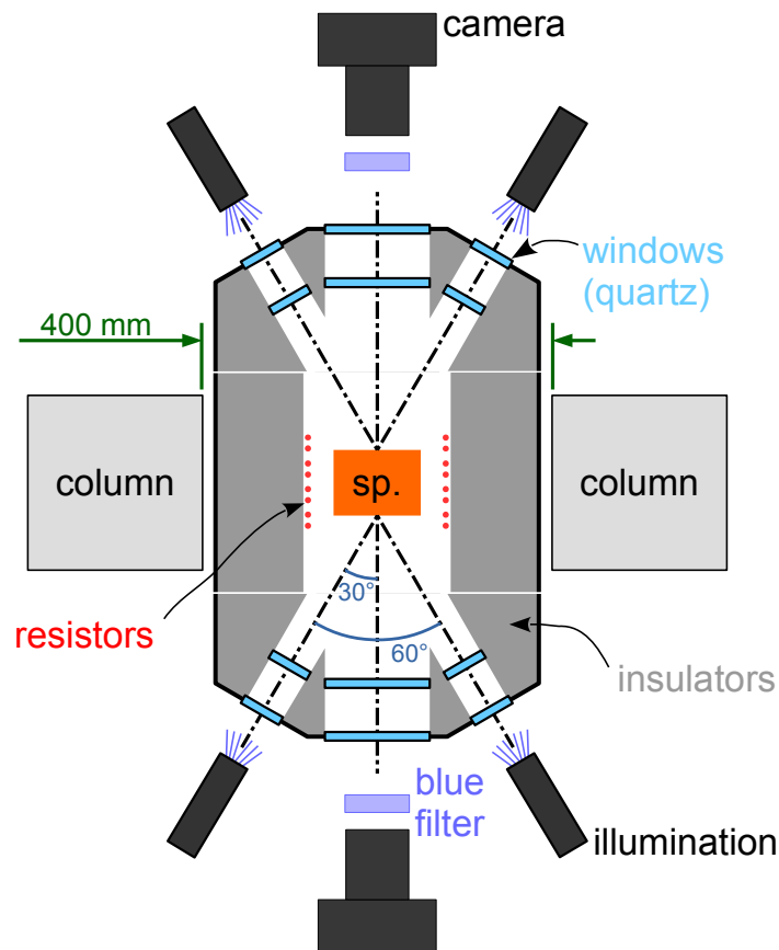
Figure 1: Top view of the furnace for up to 900°C tests displaying the setup used in the analyses presented in Section 3.
