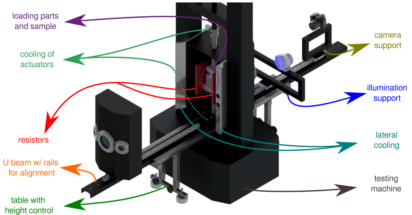
Figure 2: 3D assembly of the developed F900 setup to perform thermomechanical experiments up to 900°C.
