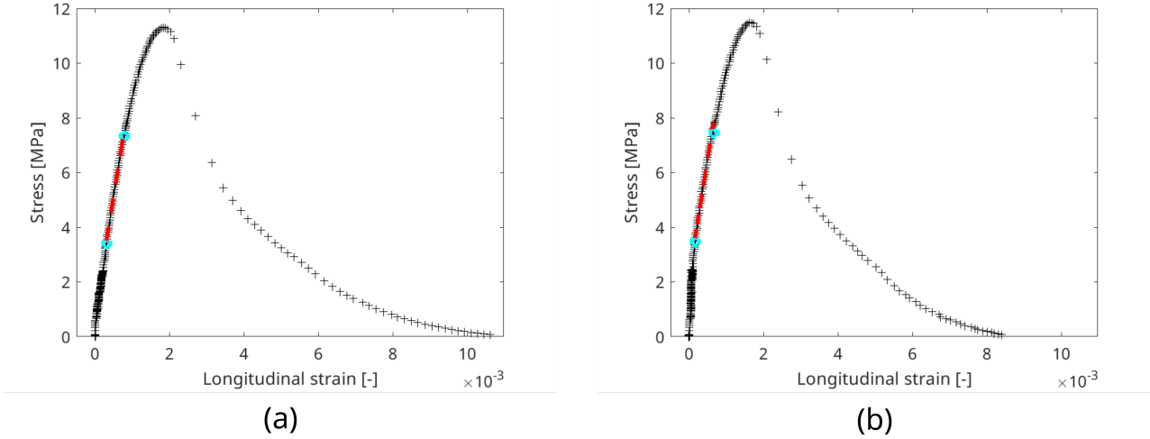
Figure 12: Maximum stress ( i.e. , at the bottom of the beam) as the respective longitudinal strain for the (a) front and (b) back analyzed surfaces. Cyan circles depict the points used for calculating the Young’s modulus (same points are highlighted in Figure 10(b)), and the respective affine slope is shown as a dashed red line.
