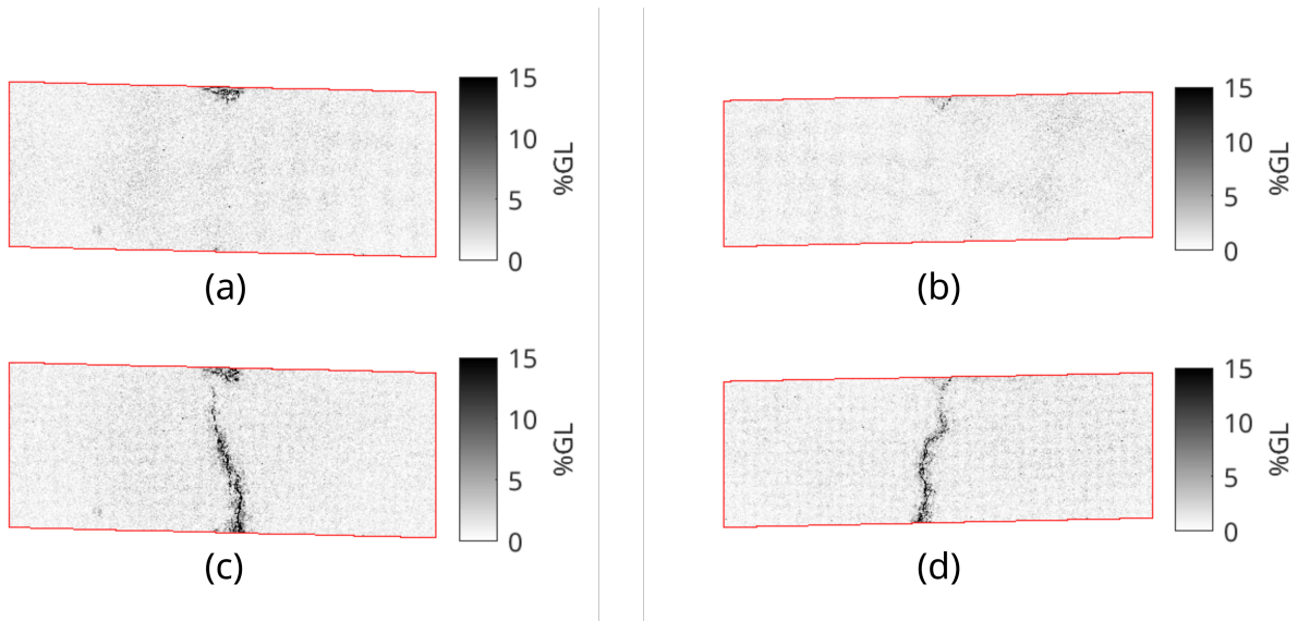
Figure 14: Absolute gray level residuals normalized by the dynamic range of the reference images for (a, b) the ultimate load and for (c,d) the last frame. Results for the front surface in sub-figures (a,c) and for the back surface in sub-figures (b,d).
