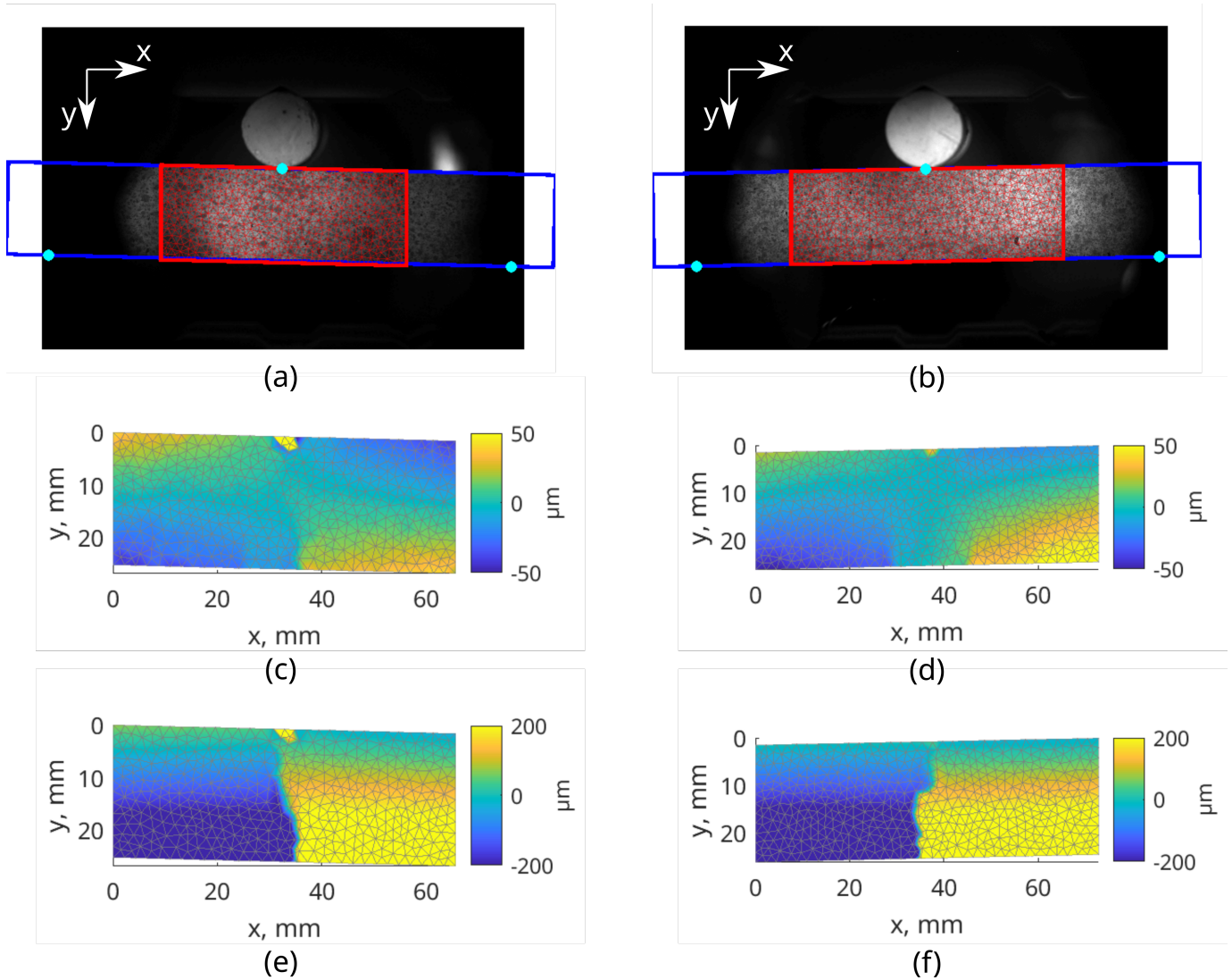
Figure 11: (a,b) Reference images with the meshes used for analyzing the three-point bend test performed at 900°C. The blue contour delineates the specimen, the red contours depict the mesh used for analyzing the more illuminated region on both sides, and the cyan circles depict the contact points of the sample with the cylinders. Horizontal displacement fields for (c,d) the time step with the maximum force and (e,f) for the last analyzed time step. Results for the front face in sub-figures (a,c,e) and for the back face in sub-figures (b,d,f). 1 px \approx 14.8 \mu\text{m} .
