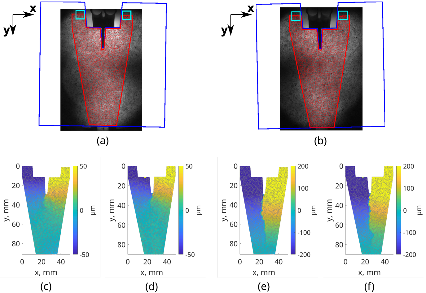
Figure 16: (a,b) Reference images with two sets of meshes used for analyzing the WST performed at 900^\circ\text{C} . The blue contour delineates the specimen, while the red one depicts the mesh used for analyzing the chosen region on both sides. Zones used to calculate the CMOD are depicted with cyan boxes. Horizontal displacement fields for (c,d) the step of the ultimate force and (e,f) the last time step. Results for the front surface in sub-figures (a,c,e) and for the back surface in sub-figures (b,d,f). 1\ \text{px} \approx 11.4\ \mu\text{m} .
