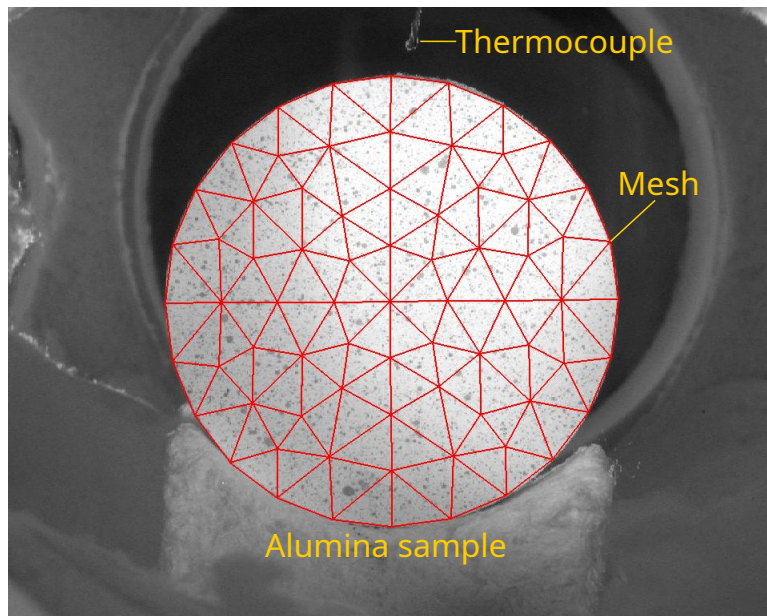
Figure B.19: Mesh used for DIC-monitored dilatometry of calcined alumina.
