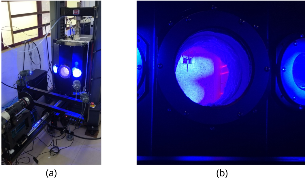
Figure 3: (a) Finalized F900 setup, with (b) a zoom on a WST specimen at 900°C
