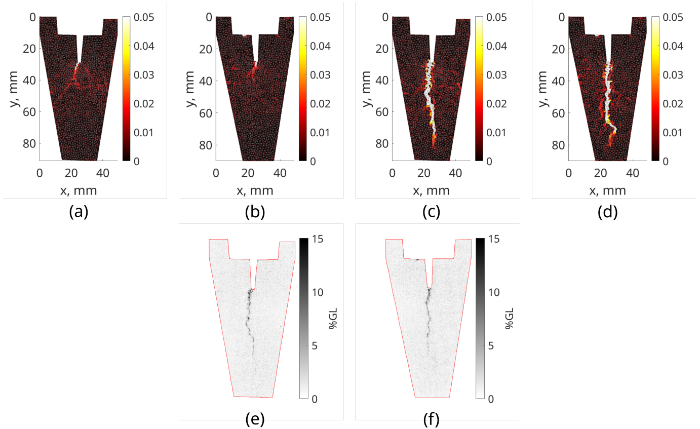
Figure 18: Maximum principal strains for (a,b) the time step of the ultimate force and (c,d) for the last time step of the WST performed at 900°C. (e,f) Absolute gray level residuals for the last analyzed time step normalized by the dynamic range of the reference images. Results for the front surface in sub-figures (a,c,e) and for the back surface in sub-figures (b,d,f).
