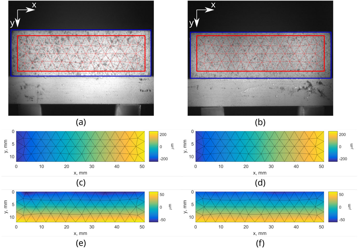
Figure 8: (a,b) Reference images with the meshes (in red) used for analyzing the YSZ specimen dilatometry up to 850°C. (c,d) Horizontal and (e,f) vertical displacement fields for the maximum temperature. Sub-figures for the front face in (a,c,e) and for the back face in (b,d,f). In the images, 1 px \approx 13.4 \mu m.
