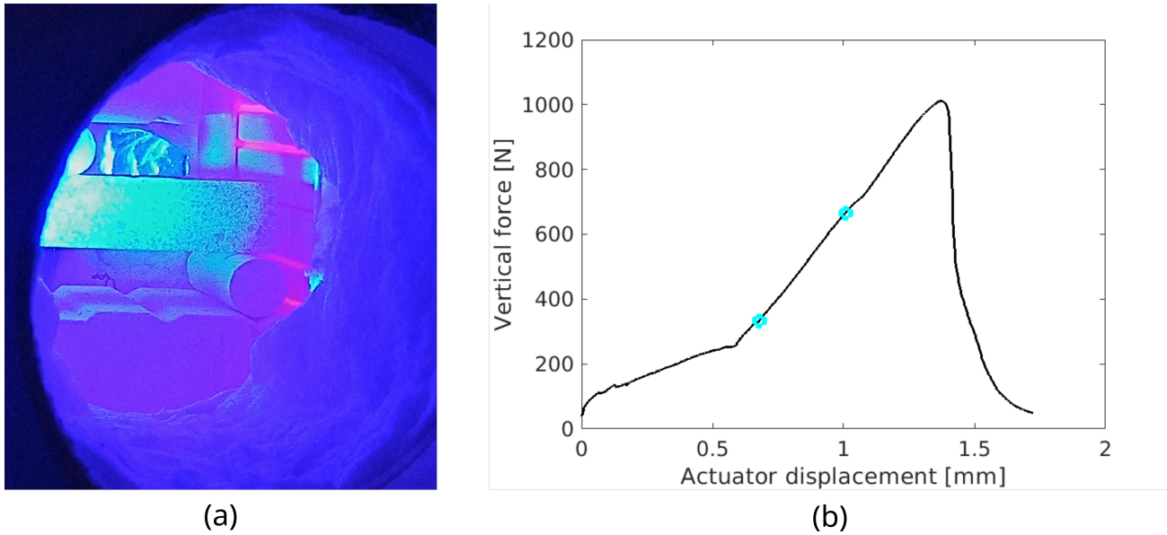
Figure 10: (a) Three-point bending sample inside the F900 furnace at 900^\circ\text{C} during the experiment. (b) Resulting loading curve. The cyan circles depict the region where the Young's modulus was calculated.
