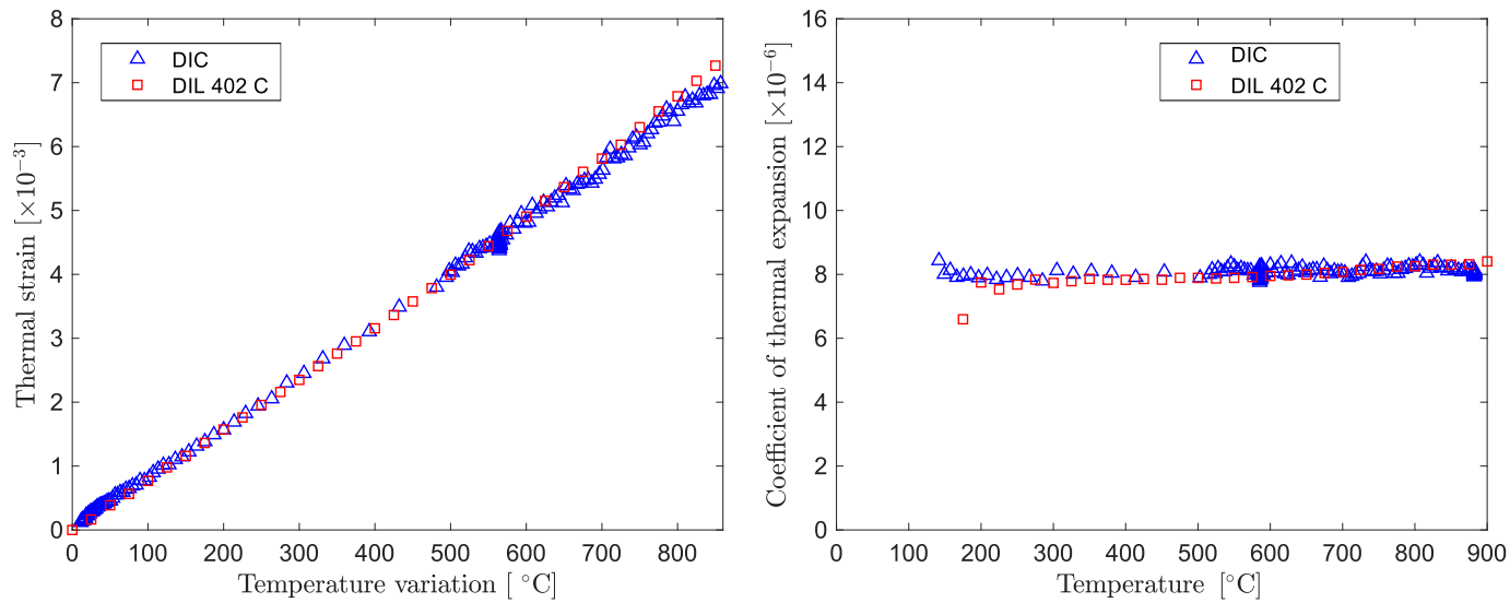
Figure B.20: DIC dilatometry validation experiments. Comparison of data with DIL 402C push-rod dilatometer for a calcined alumina specimen.
