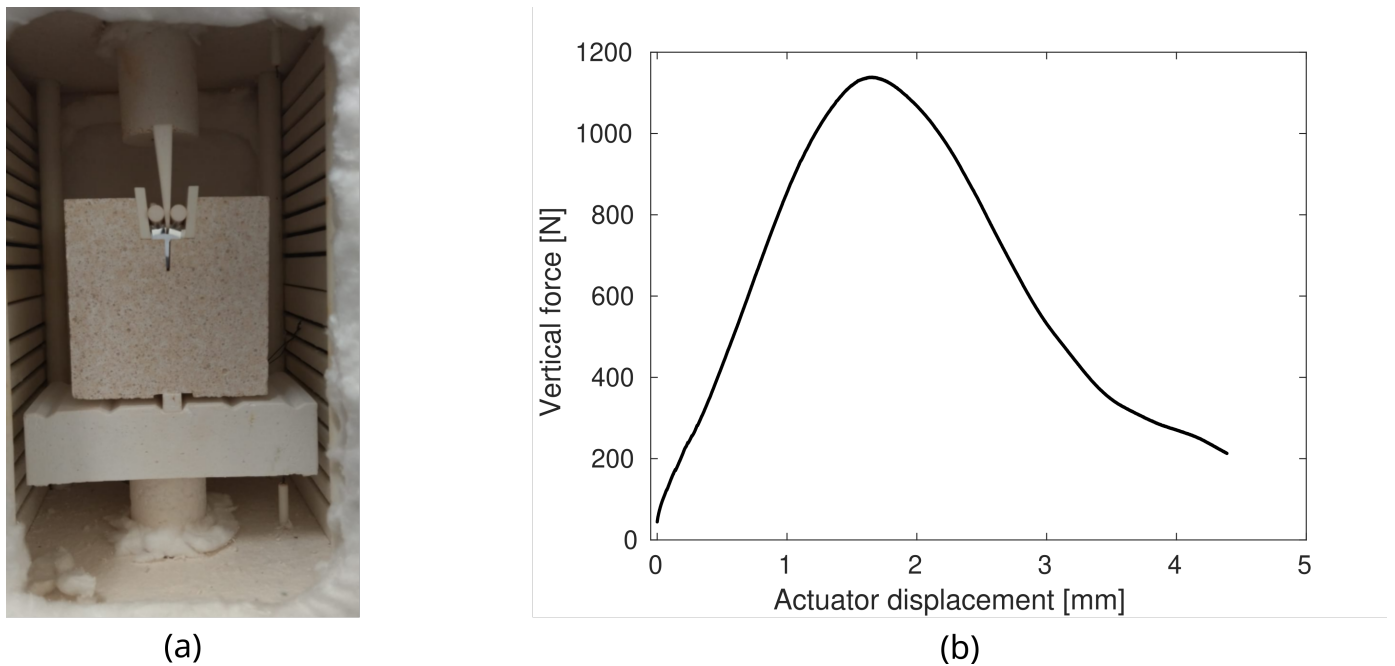
Figure 15: (a) Post-mortem wedge splitting test sample inside the F900 furnace. (b) Loading curve obtained with the 900°C setup
