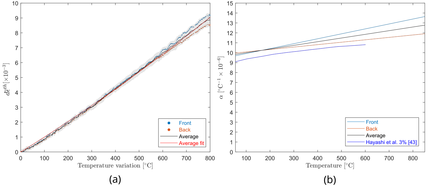
Figure 9: Dilatometry test conducted in the F900 furnace for a YZS specimen. (a) Thermal strain computed for DIC results with images of the two opposite faces of the specimen and its average value. A second-degree polynomial interpolates the thermal strain average to allow for the computation of the differential CTE. The gray patch shows the standard strain uncertainties. (b) Differential CTE \alpha obtained from the DIC analyses of opposite sides of the specimen. The average of them is compared with literature results [43].
