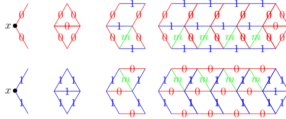
FIGURE 13. First row from left to right : an opening a with color 0 and type 0 at x , the case C(e'') = c , the case C(e'') \neq c and an arrow of length r = 4 . The second row is the analog for color 1. Uncolored edges have color 3.
