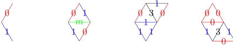
FIGURE 21. A 01 opening (left) and its possible completions
