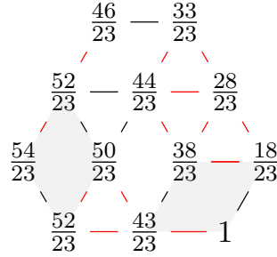
FIGURE 5. A toric rhombus concave function for n = 3, d = 1 : the regular labeling is depicted through colored edges and the shaded lozenge are the rigid ones yielding the equality cases in the toric rhombus concavity.
