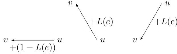
FIGURE 28. Values at vertices when traversing an edge e = (u, v) .
