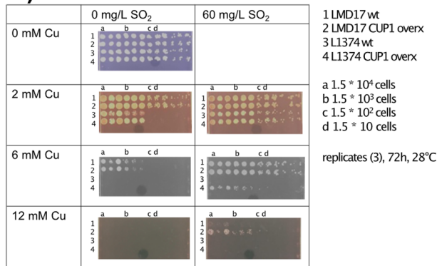
Figure 5. Effect of SO 2 addition in the media on copper resistance. (A) Resistance of oak strain Oak-Rom 3.2 to copper (0 to 1 mM) in the absence (control) and presence of 40 mg/L SO 2 . (B) Resistance of wine strain LMD17 and L1374 to copper (0 to 12 mM) in the absence (control) and presence of SO 2 (60 mg/L).
