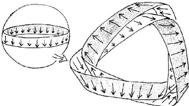
Fig.2 : How the coincidence of antipodal regions creates T-symmetry.
