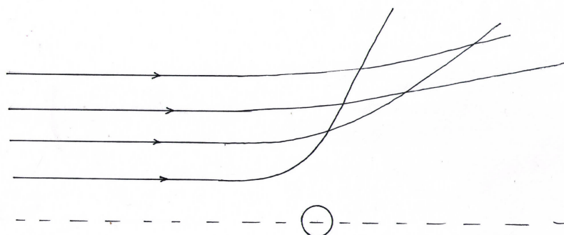
Fig.6 Geodesics created by negative mass.
