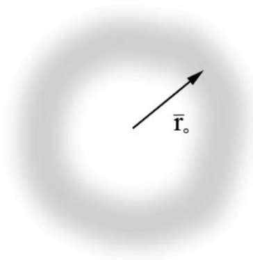
Fig.13 – Attenuation of the magnitude of objects in the background of the dipole repeller
