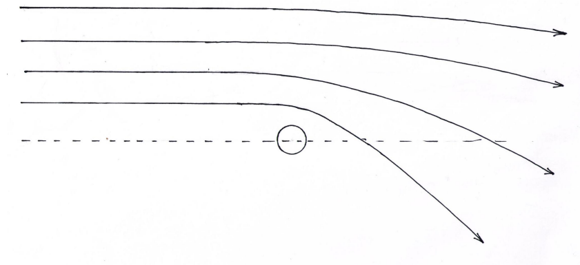
Fig.5 Geodesics created by a positive mass.
