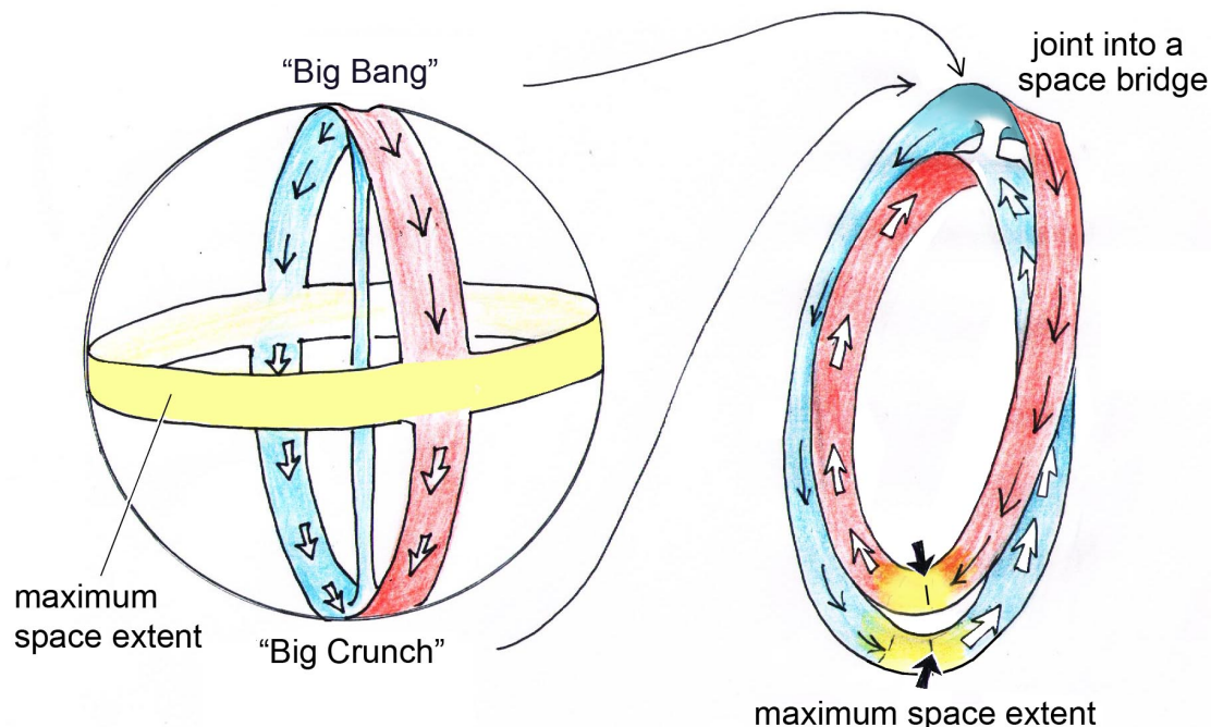
Fig.3 : Coincidence of antipodal regions on a sphere S^2 , according to the two-folds cover of a half-turn Möbius strip, with the appearance of T-symmetry.
