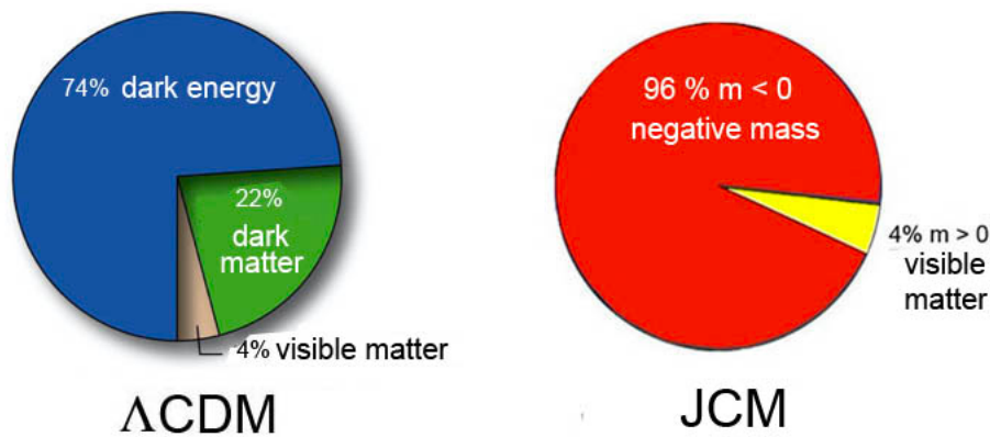
Fig.9 : Comparative contents of the \Lambda CDM and Janus models :
