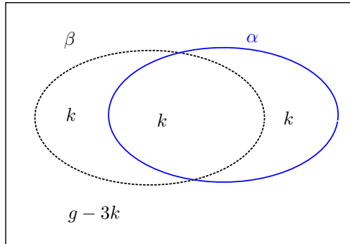
FIGURE 2. The images of the Dehn twists \tau_\alpha and \tau_\beta by \rho_{1,k} commute
