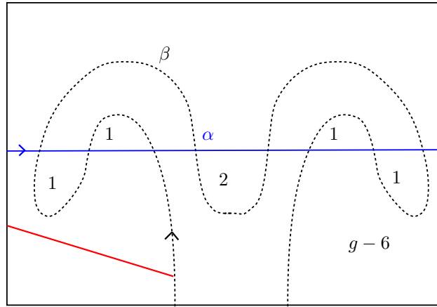
FIGURE 1. Two disjoint arcs on which the intersection form \langle\cdot, \cdot\rangle_{\mathbb{H}_g} vanishes. The surface \Sigma_{g,1} is represented by a square with handles added. If a region is colored by an integer k , it means that one needs to add k handles in that region. In red, the thread for \beta is represented.
