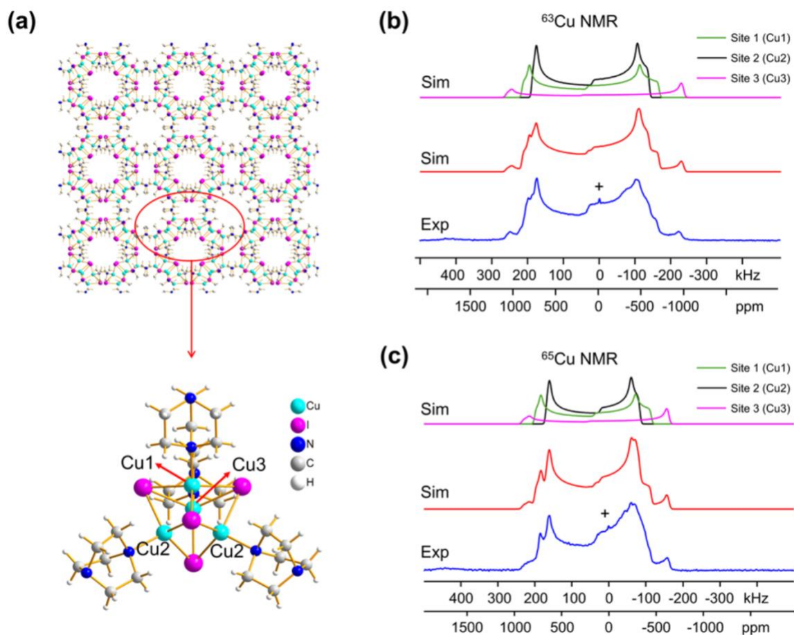
Figure 1: A schematic diagram of [Cu 4 I 4 (DABCO) 2 ] featuring three different Cu sites. The experimental (b) 63 Cu and (c) 65 Cu static NMR spectra (blue), cumulative simulations (red), and individual Cu site simulations (black, purple, green).
