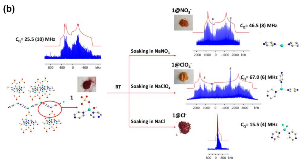
Figure 2: (a) The relation between the chemical environment of Cu (I) and their C_Q values. (b) The obvious change in linewidth and C_Q indicate a possible structural change of (\text{Cu}_2(\text{SO}_4)(\text{pyz})_2(\text{H}_2\text{O})_2) upon addition of various aqueous solutions.
