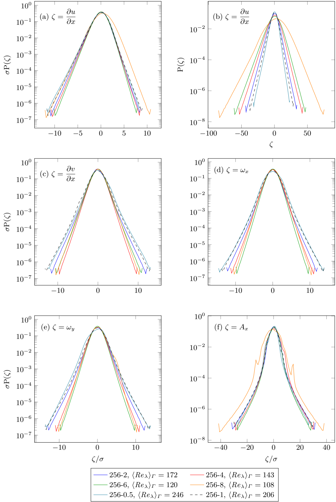
FIG. 9: \zeta -PDFs for (a), (b) \zeta = \partial u/\partial x , (c) \zeta = \partial v/\partial x , (d) \zeta = \omega_x , (e) \zeta = \omega_y , (f) \zeta = A_x (Lagrangian acceleration), averaged over the study time interval \Gamma of variable-density simulations, and compared with the constant-density initial condition (dashed). DNS parameters are listed in table I. \sigma is the standard deviation of \zeta in each PDF. \langle Re_\lambda \rangle represents the averaged turbulent Reynolds number over time interval \Gamma . In (b), the PDF has not been normalized by \sigma .
