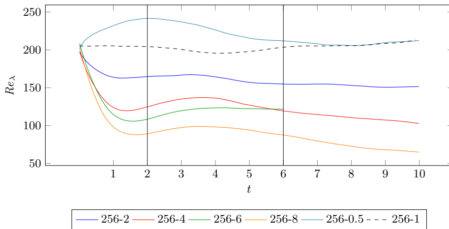
FIG. 8: Time evolution of the turbulent Reynolds number Re_\lambda = (\lambda/L) Re during variable-density simulations. DNS parameters are listed in table I. For comparison, dashed line depicts the evolution throughout constant-density simulation 256-1 for t \in [40, 50] . Vertical lines delimit the study time interval \Gamma which is considered for the statistical computations.
