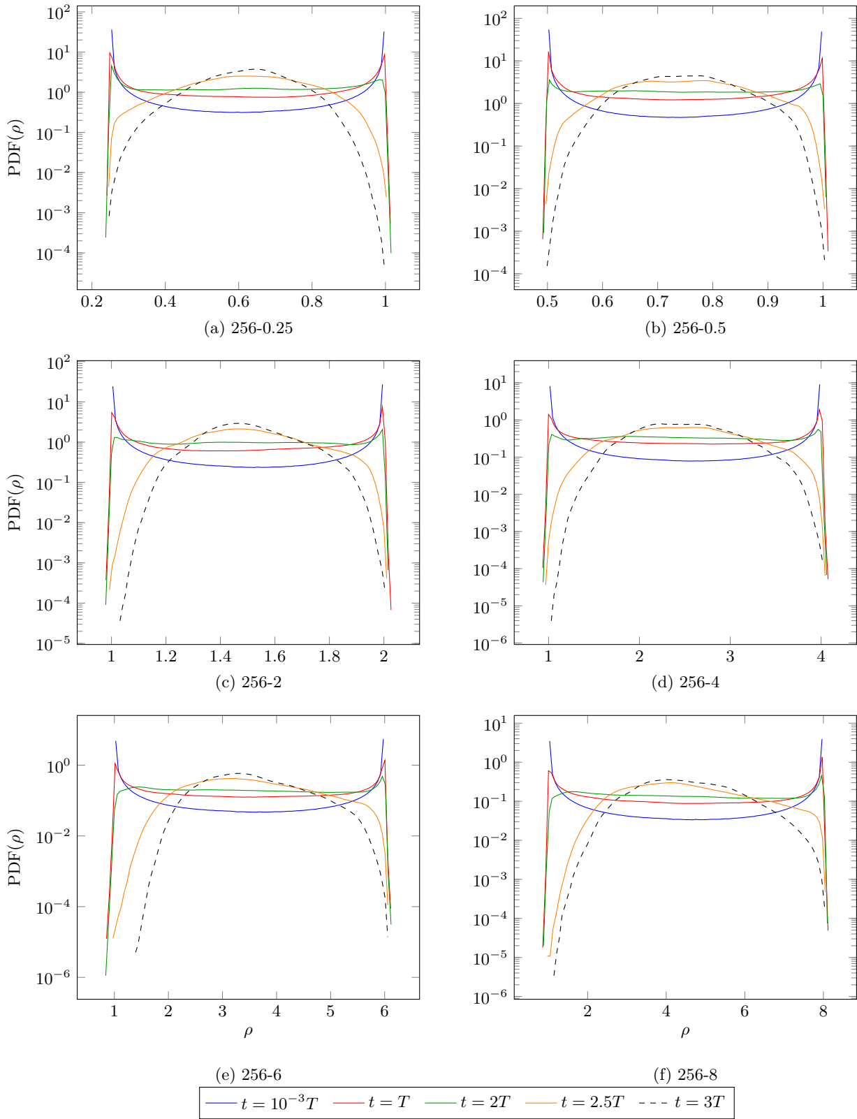
FIG. 4: Density field PDF evolution during DNSs of variable-density HIT. Simulation parameters for variable-density HIT DNSs are listed in table I page 5.
