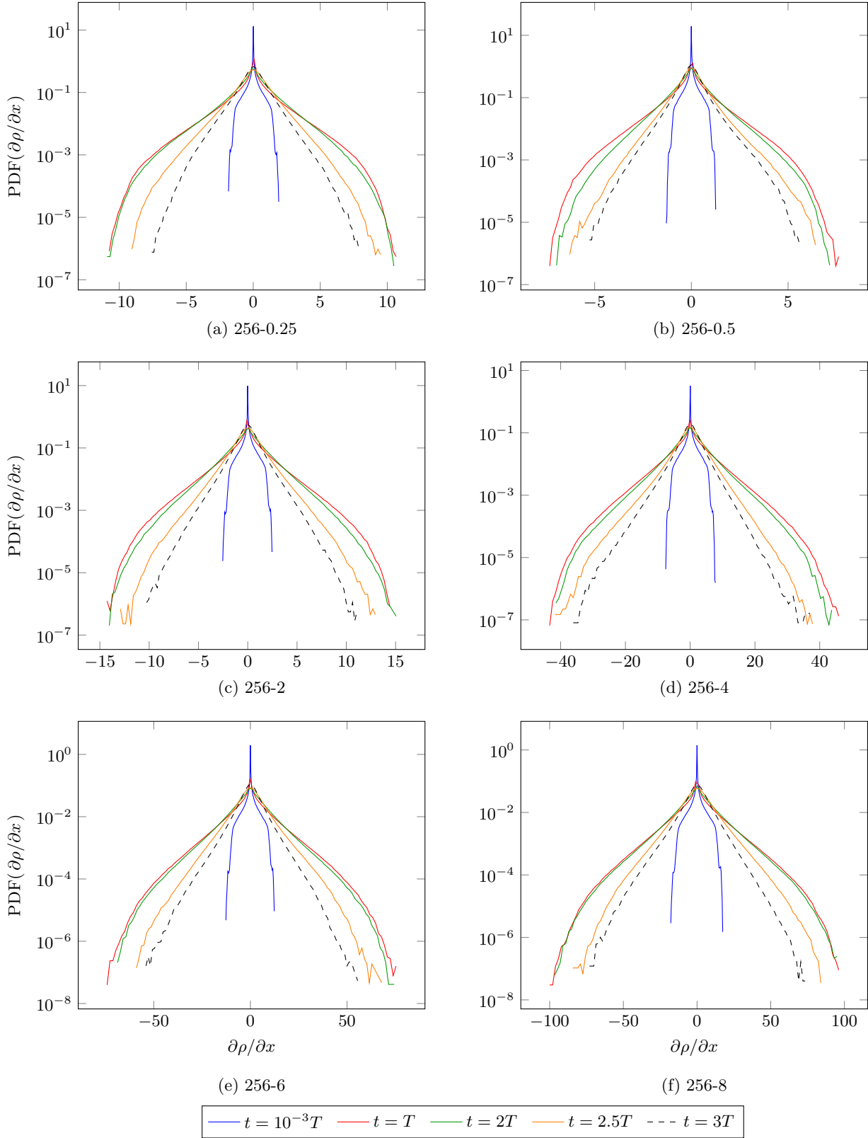
FIG. 6: \partial\rho/\partial x PDF evolution during DNSs of variable-density HIT. Simulation parameters for variable-density HIT DNSs are listed in table I page 5.
