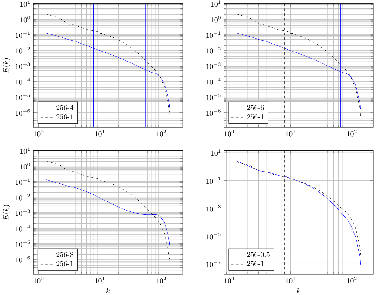
FIG. 14: Spectra averaged over the study time interval \Gamma of variable-density simulations, and compared with the constant-density initial condition (dashed). The vertical lines represent the integral and Taylor scales associated with the equations defined in eqs. (16) and (17). Simulation parameters for variable-density HIT DNSs are listed in table I page 5.
