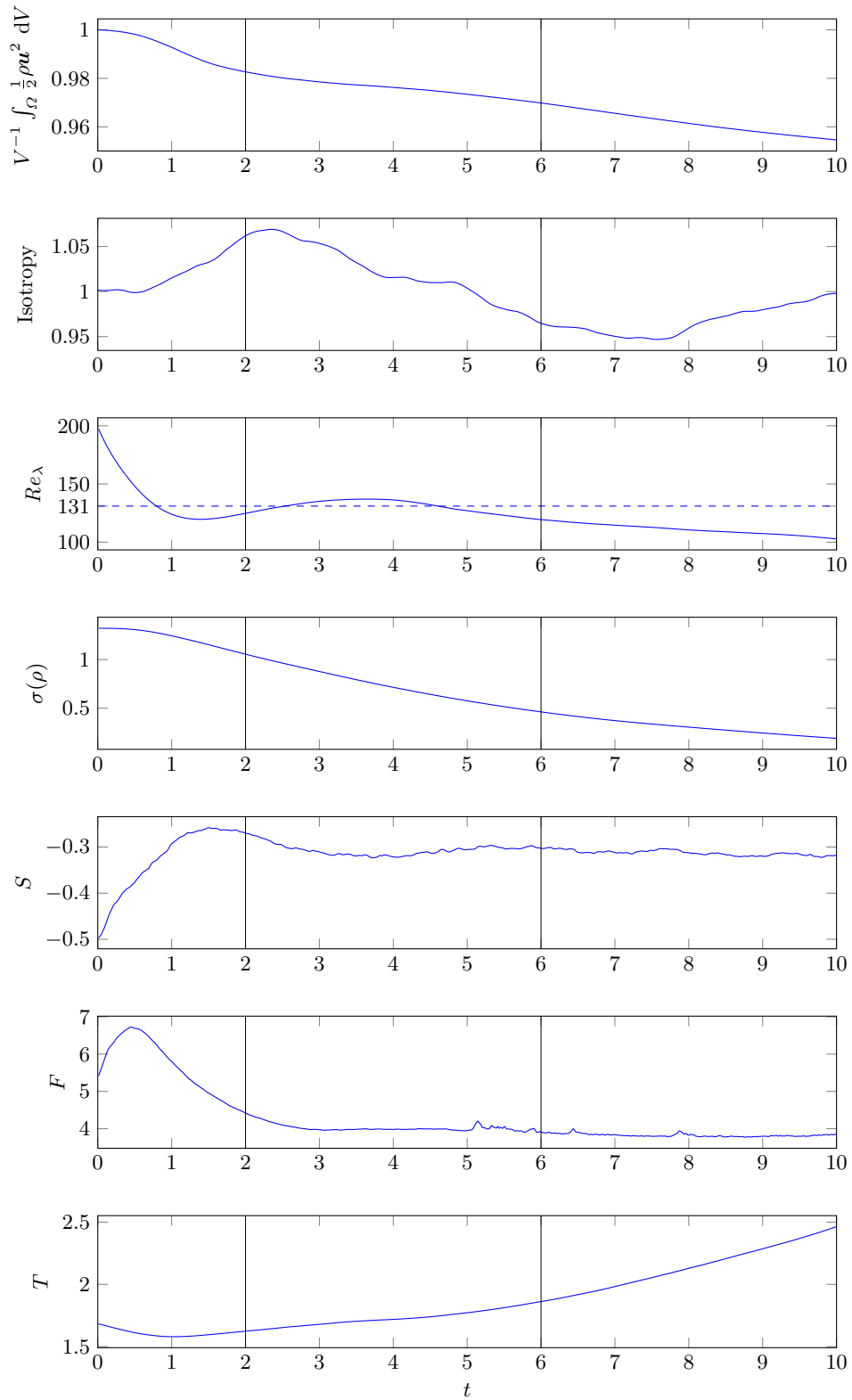
FIG. 3: Evolution of the volumetric total kinetic energy, isotropy degree [33] (calculation detailed in appendix B), microscale Reynolds number Re_{\lambda} , density field standard deviation in space \sigma(\rho) , velocity longitudinal-derivative skewness S , and eddy turnover time T during simulation run 256-4. Vertical lines delimit a time interval T of 2 eddy turnover times, where turbulent parameters do not fluctuate much, and where mass diffusion effects are still significant. Re = 1000 , s = 4 , Sc = 1 , N = 256 .
