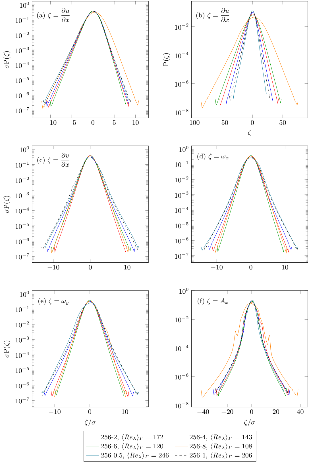
FIG. 9: \zeta -PDFs for (a), (b) \zeta = \partial u / \partial x , (c) \zeta = \partial v / \partial x , (d) \zeta = \omega_x , (e) \zeta = \omega_y , (f) \zeta = A_x (Lagrangian acceleration), averaged over the study time interval \Gamma of variable-density simulations, and compared with the constant-density initial condition (dashed). DNS parameters are listed in table I. \sigma is the standard deviation of \zeta in each PDF. \langle Re_\lambda \rangle represents the averaged turbulent Reynolds number over time interval \Gamma . In (b), the PDF has not been normalized by \sigma .
