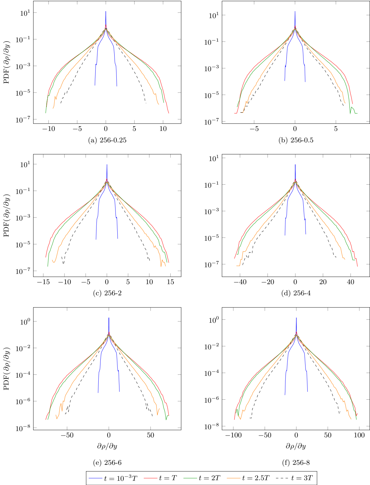
FIG. 7: \partial\rho/\partial y PDF evolution during DNSs of variable-density HIT. Simulation parameters for variable-density HIT DNSs are listed in table I page 5.
