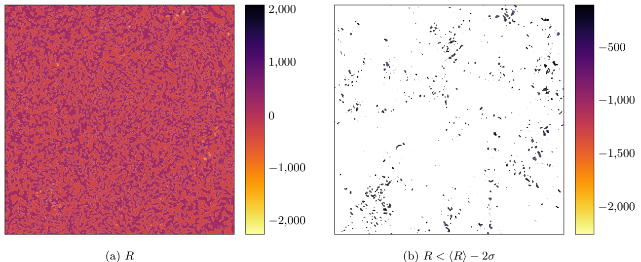
FIG. 15: xz -Cross-section plot of the Rayleigh–Taylor instability criterion ( R ) at time t = 4 of simulation 256-4. Re = 1000 , s = 4 , Sc = 1 , N = 256 .
