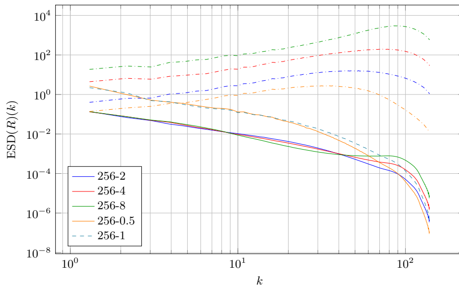
FIG. 16: Spectra averaged over the study time interval T of variable-density simulations, and compared with the spectral density of the Rayleigh–Taylor instability criterion R (dotted). DNS parameters are listed in table I.
