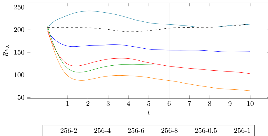
FIG. 8: Time evolution of the turbulent Reynolds number Re_\lambda = (\lambda/L) Re during variable-density simulations. DNS parameters are listed in table I. For comparison, dashed line depicts the evolution throughout constant-density simulation 256-1 for t \in [40, 50] . Vertical lines delimit the study time interval \Gamma which is considered for the statistical computations.
