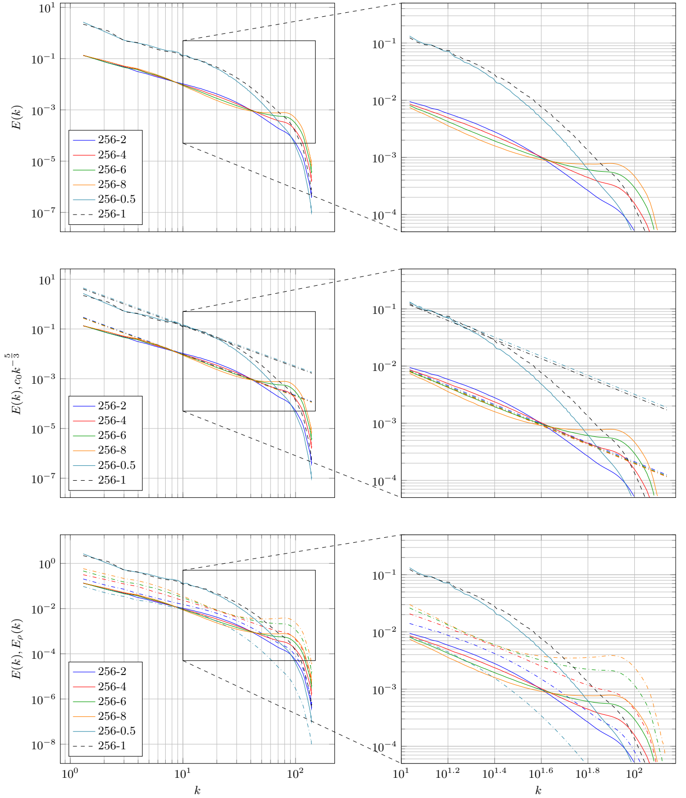
FIG. 12: Spectra averaged over the study time interval T of variable-density simulations, and compared with the constant-density initial condition (dashed). Simulation parameters for variable-density HIT DNSs are listed in table I page 5.
