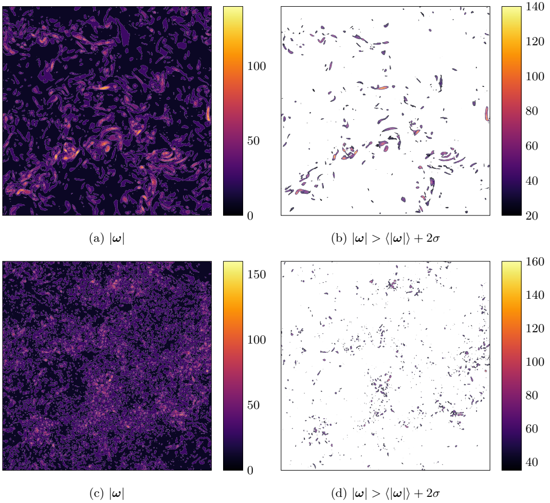
FIG. 11: xz -Cross-section plot of the vorticity norm for both (a), (b) the constant-density initial condition and (c), (d) the variable-density simulation 256-4 (at time t = 4 ). Re = 1000 , s = 4 , Sc = 1 , N = 256 .
