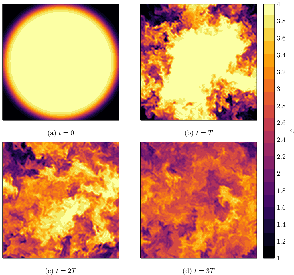
FIG. 2: xz -Cross-section plot of the density field at different times during simulation run 256-4. Re = 1000 , s = 4 , Sc = 1 , N = 256 .
