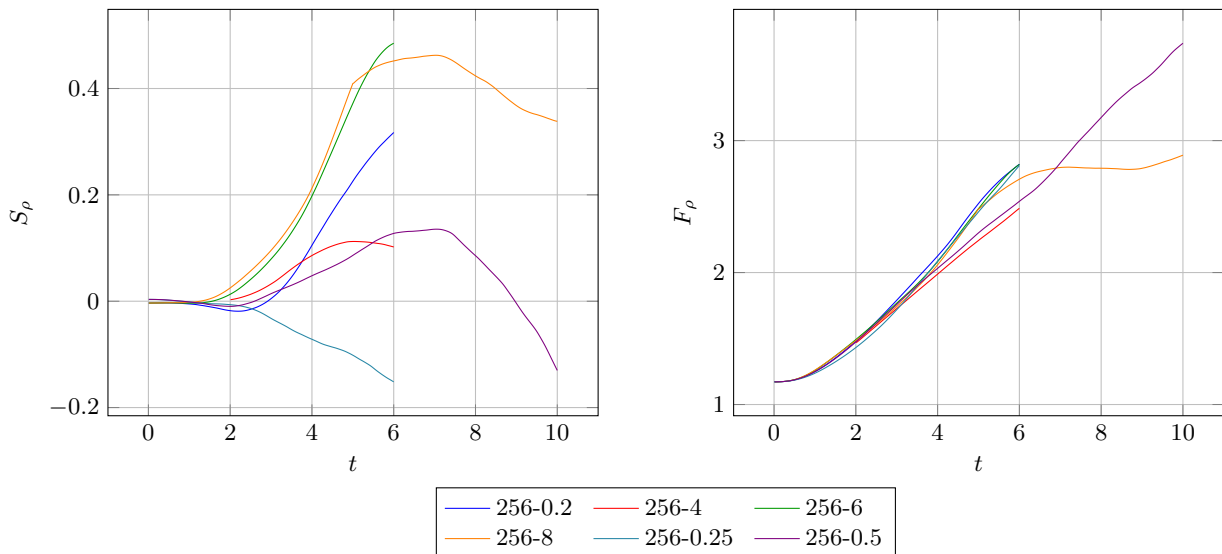
FIG. 5: Density field moments evolution during DNSs of variable-density HIT: (left) skewness defined in eq. (19) ; (right) flatness defined in eq. (20). Simulation parameters for variable-density HIT DNSs are listed in table I page 5.
