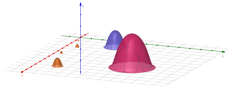
Figure 1: Sketch of the function constructed in Lemma 3.9.
