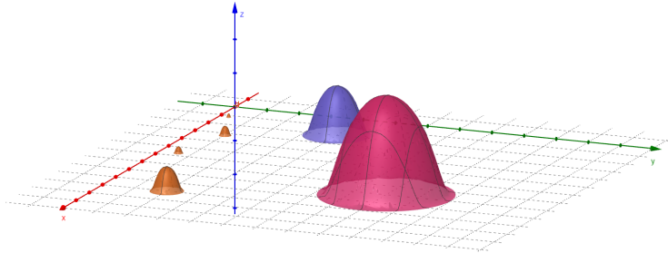
Figure 1: Sketch of the function constructed in Lemma 3.9.
