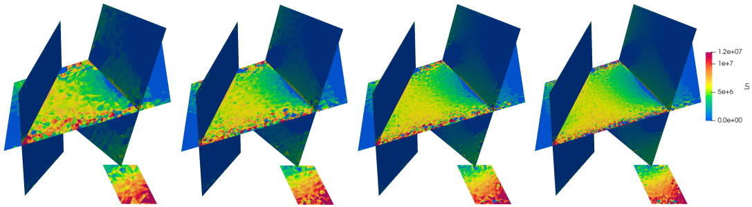
Figure 6. Normal surface traction \lambda on the fracture network obtained with the four meshes with from left to right 47k, 127k, 250k and 450k cells.
