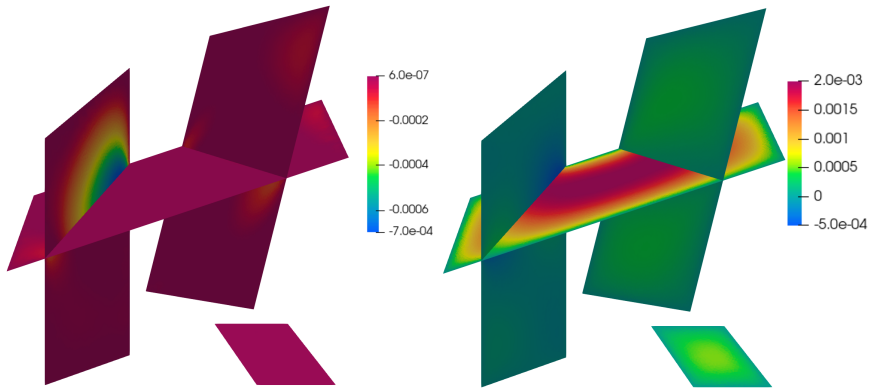
Figure 4. Normal (left) and \tau_2 -tangential (right) jumps along the fracture network obtained on the finest mesh with 450k cells.
