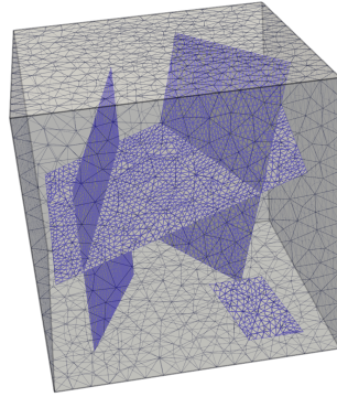
Figure 3. Polytopal mesh of the 3D DFM with roughly 47k cells and 6k fracture faces and obtained from an initial tetrahedral mesh refined along the fracture network by cutting each fracture face in four triangle.
