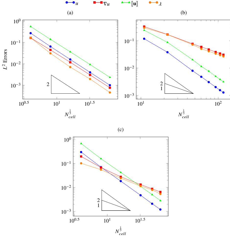
Figure 2. Relative L^2 norms of the errors \mathbf{u} - \Pi^{\mathcal{D}}\mathbf{u}_{\mathcal{D}} , [\mathbf{u}] - [[\mathbf{u}_{\mathcal{D}}]]_{\mathcal{D}} , \nabla\mathbf{u} - \nabla^{\mathcal{D}}\mathbf{u}_{\mathcal{D}} and \lambda - \lambda_{\mathcal{D}} as a function of the cubic root of the number of cells, using the families of Cartesian (a), tetrahedral (b) and hexahedral (c) meshes.
