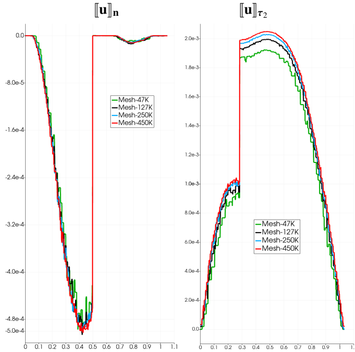
Figure 5. For the four meshes, plot over line along the diagonal of the left vertical fracture for the normal jump (left) and along the diagonal of the almost horizontal fracture for the \tau_2 -tangential jump (right).
