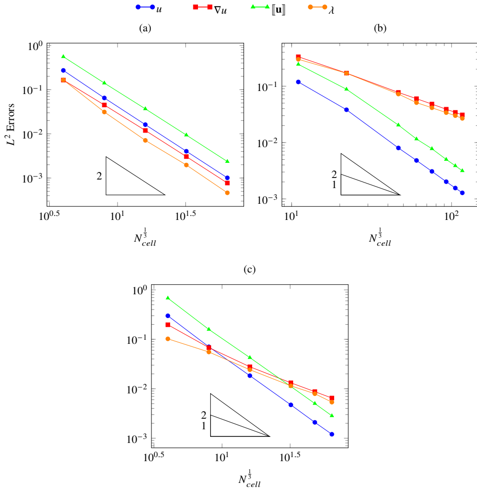
Figure 3: Relative L^2 norms of the errors \mathbf{u} - \Pi^{\mathcal{D}}\mathbf{u}_{\mathcal{D}} , \llbracket \mathbf{u} \rrbracket - \llbracket \mathbf{u}_{\mathcal{D}} \rrbracket_{\mathcal{D}} , \nabla \mathbf{u} - \nabla^{\mathcal{D}}\mathbf{u}_{\mathcal{D}} and \lambda - \lambda_{\mathcal{D}} as a function of the cubic root of the number of cells, using the families of Cartesian (a), tetrahedral (b) and hexahedral (c) meshes.
