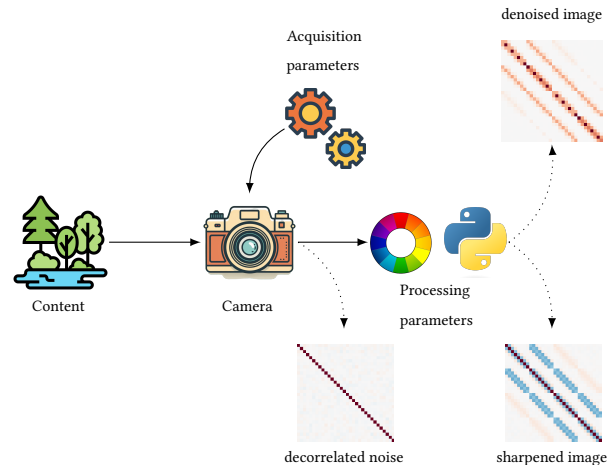
Figure 1: Schematic reasoning for the multivariate distribution of the noise in natural images. 1
