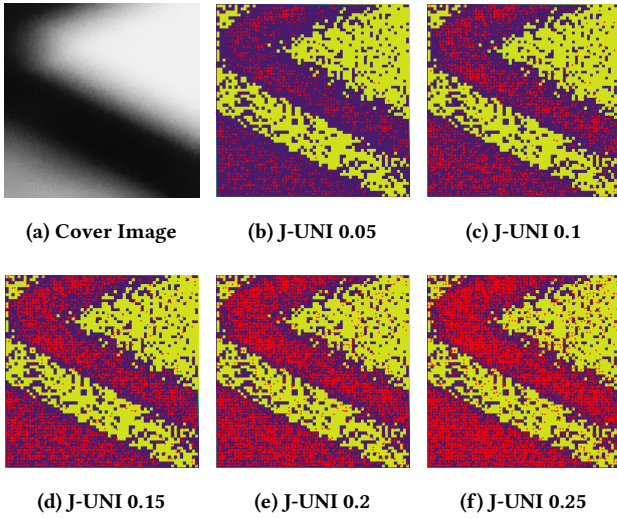
Figure 2: Sampling strategy against adaptive embedding strategy (J-uniward): (a) cover image, (b)-(f) embeddings at 0.05, 0.1, 0.15, 0.2, 0.25 bpnzAC respectively. Yellow and purple areas indicate the selected and rejected samples for the correlation estimation, respectively. The red dots indicate the DCT coefficients modified with the embedding.
