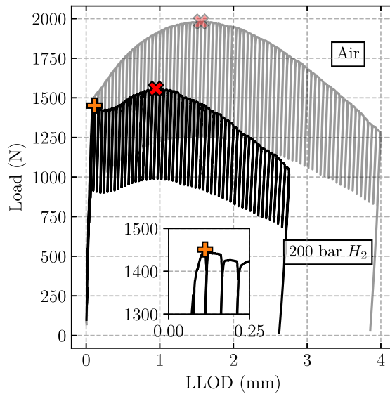
(c) Load – LLOD plot.
