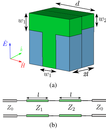
Fig. 6. Simulation setup to test the validity of the model (a) Two T-shape unit cells together; d = 2.7 mm, l = 1 mm, w_1 = 0.9 mm, w_2 = 0.7 mm (b) Equivalent circuit of the two unit cells arranged, Z_1 = 279.2\Omega , Z_2 = 293.5\Omega .
