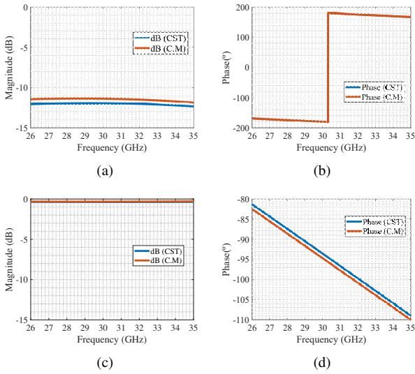
Fig. 7. Scattering parameters for the cascade of two T-shaped unit cells (a) Magnitude of the reflection coefficient in dB (b) Phase of the reflection coefficient. (c) Magnitude of the transmission coefficient in dB (d) Phase of the transmission coefficient. The range of frequency is chosen around \lambda/2 to show the most interesting results.
