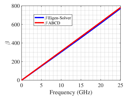
Fig. 3. Comparison between ABCD method and eigensolver for the square-shaped dielectric unit cell with a filling factor of 80% and a permittivity of 5.
