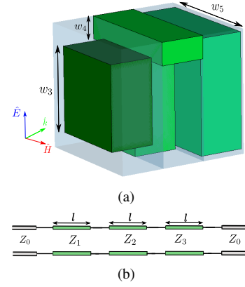
Fig. 8. Simulation setup to test the validity of the model (a) Three cells together: Square - T-shape - Square; w_3 = 1.87 mm, w_4 = 0.5 mm, w_5 = 2.53 mm. l = 1 mm (b) Equivalent circuit of the three unit cells arranged, Z_1 = 289.6\Omega , Z_2 = 252.7\Omega , Z_3 = 137.2\Omega .
