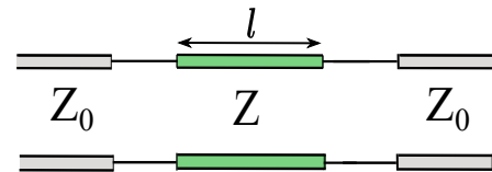
Fig. 2. Circuit model for the dielectric unit cell with length l
