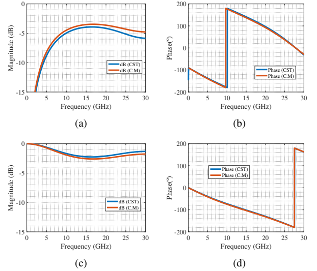
Fig. 9. Scattering parameters for the cascade of two square cells and T-shaped unit cells (a) Magnitude of the reflection coefficient in dB (b) Phase of the reflection coefficient. (c) Magnitude of the transmission coefficient in dB (d) Phase of the transmission coefficient. The range of frequency is chosen around \lambda/2 to show the most interesting results.
